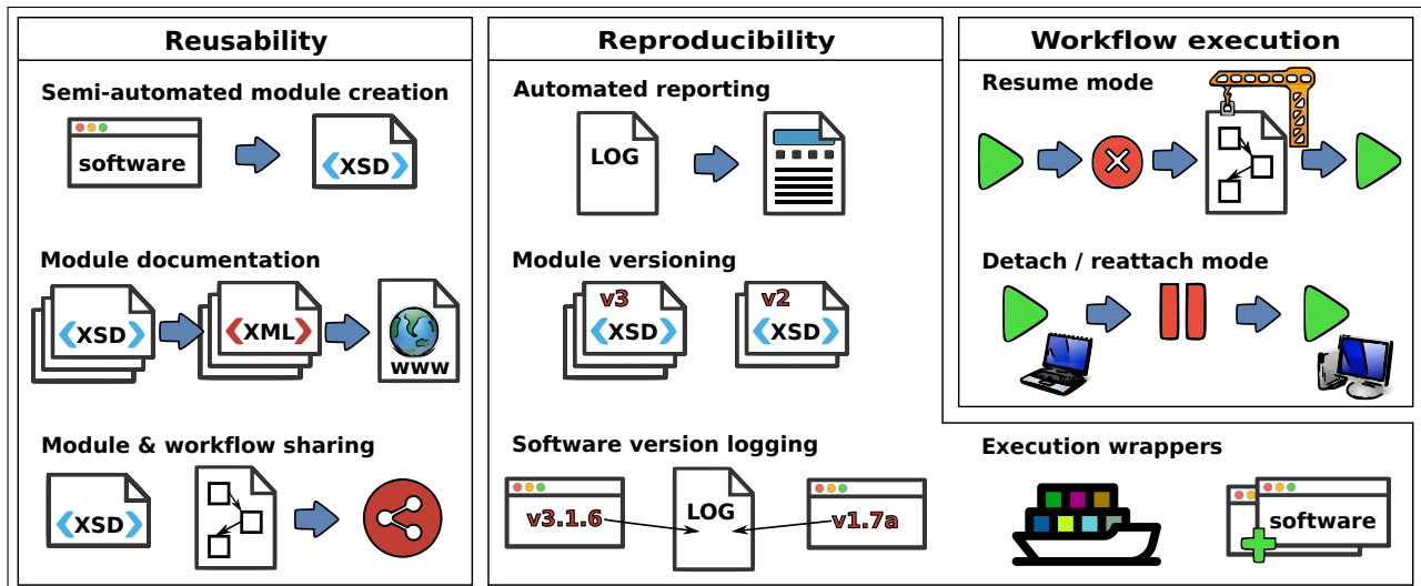
Figure 1. Overview on new developments in Watchdog 2.0 . New features are broadly grouped into the categories reusability, reproducibility, and workflow execution. Left: New modules can now be developed in a semi-automated manner from software help pages using a GUI. A standardized documentation format was developed, allowing to automatically compile a reference book of available modules. Public repositories for sharing modules and workflows are now available. Center: Extensive logging of workflow execution ensures reproducibility of results and allows automated creation of a step-by-step report on analysis methods. Versioning of modules allows adaption to new requirements with backward compatibility without unnecessary module duplication. Software and module versions are now automatically reported in the log files. Execution wrappers now allow automatic deployment of software using container virtualization or package managers. Right: Workflow execution becomes more flexible with the resume and detach/reattach modes. The resume mode allows resuming interrupted or modified workflow execution without unnecessarily re-running tasks. Detach/reattach allows shutting down the scheduler on the local host while still running tasks on a computer cluster and reattaching to workflow execution on the same or different computer at a later time.
