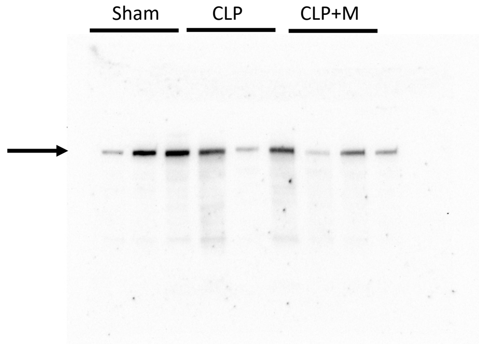
NLRP3 Blot
