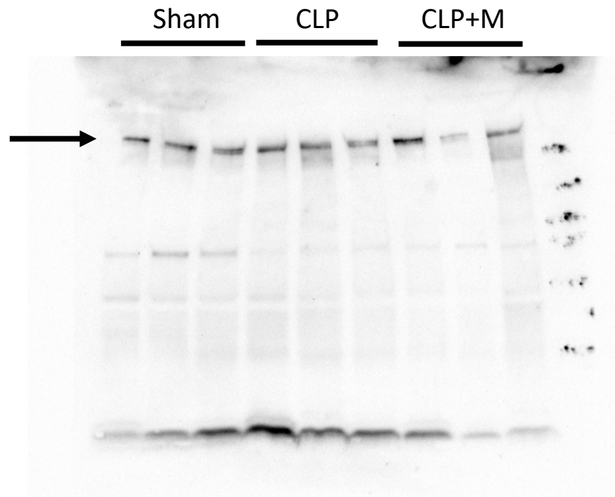
NLRP3 Blot
