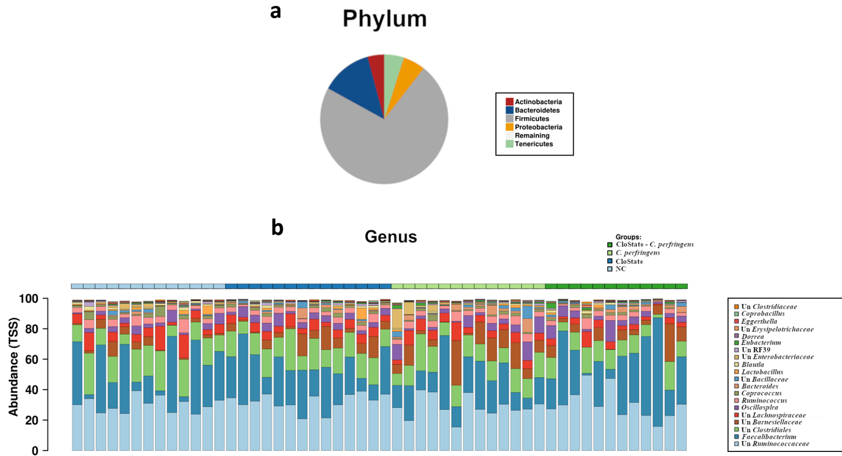
Fig. S1: Cecal microbiota composition of broilers within different groups; (A) the most dominant phyla, and (B) the 20 most abundant genera.
