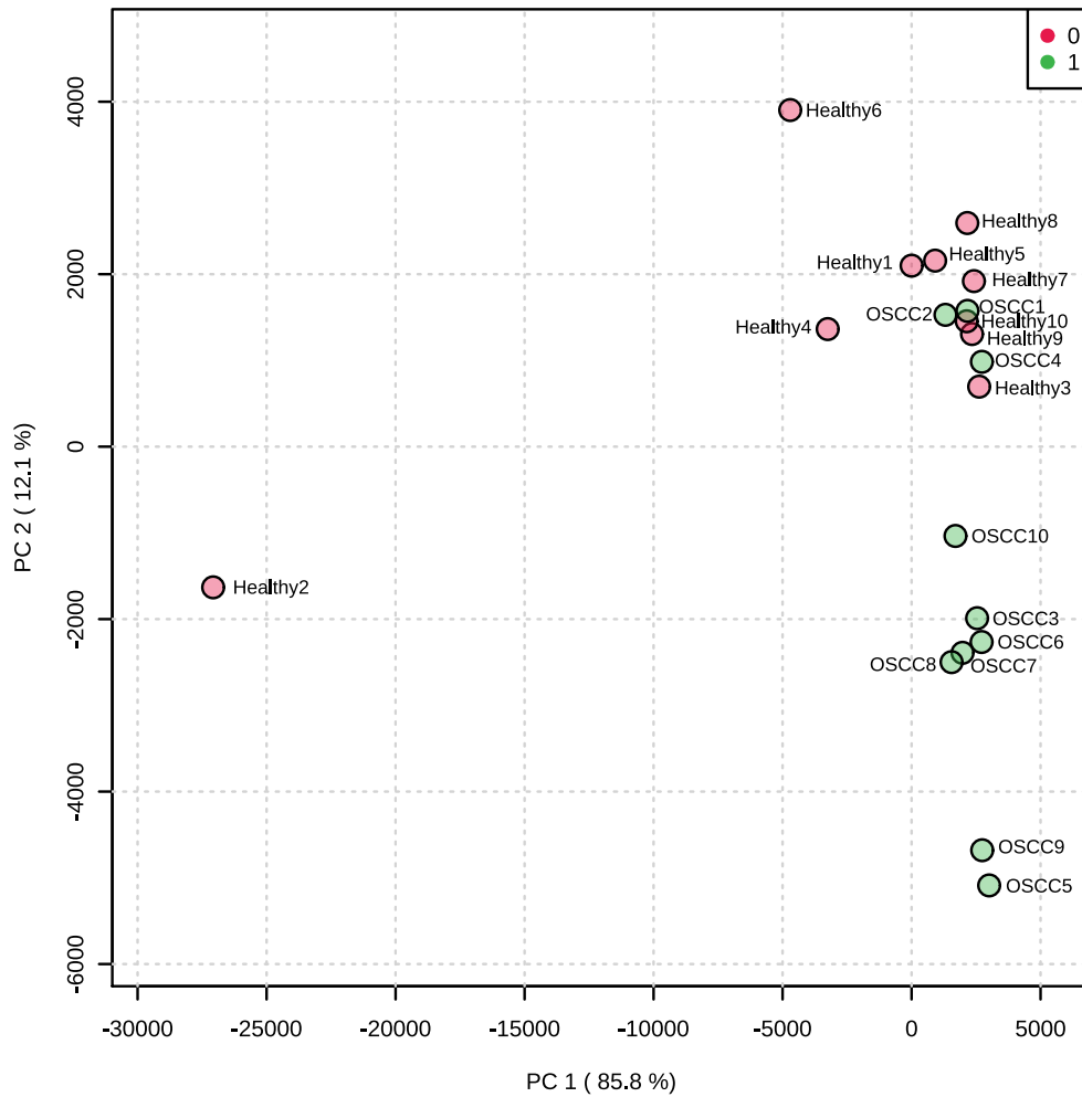
Scores Plot
