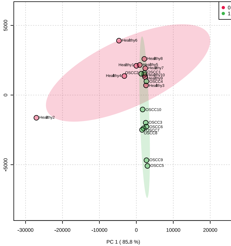
Scores Plot
