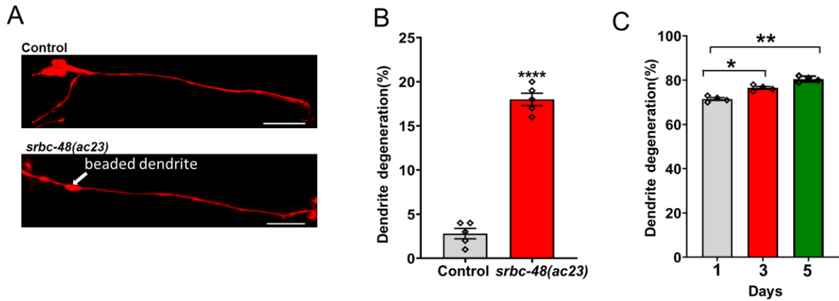
Figure S2. Early infection can lead to dendrite degeneration later in life in srbc-48(ac23) animals.
