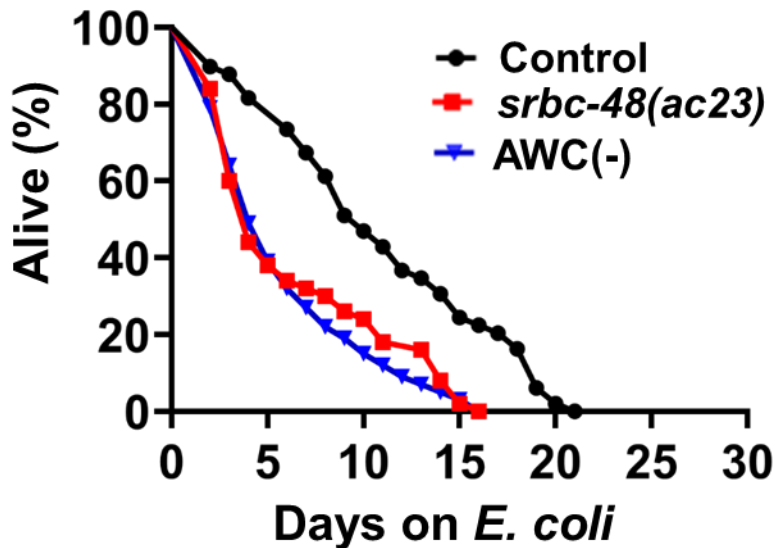
Figure S3. AWC neurons control the lifespan of the animals.
