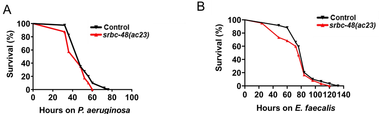
Figure S4. srbc-48(ac23) animals are not susceptible to pathogen-mediated killing
