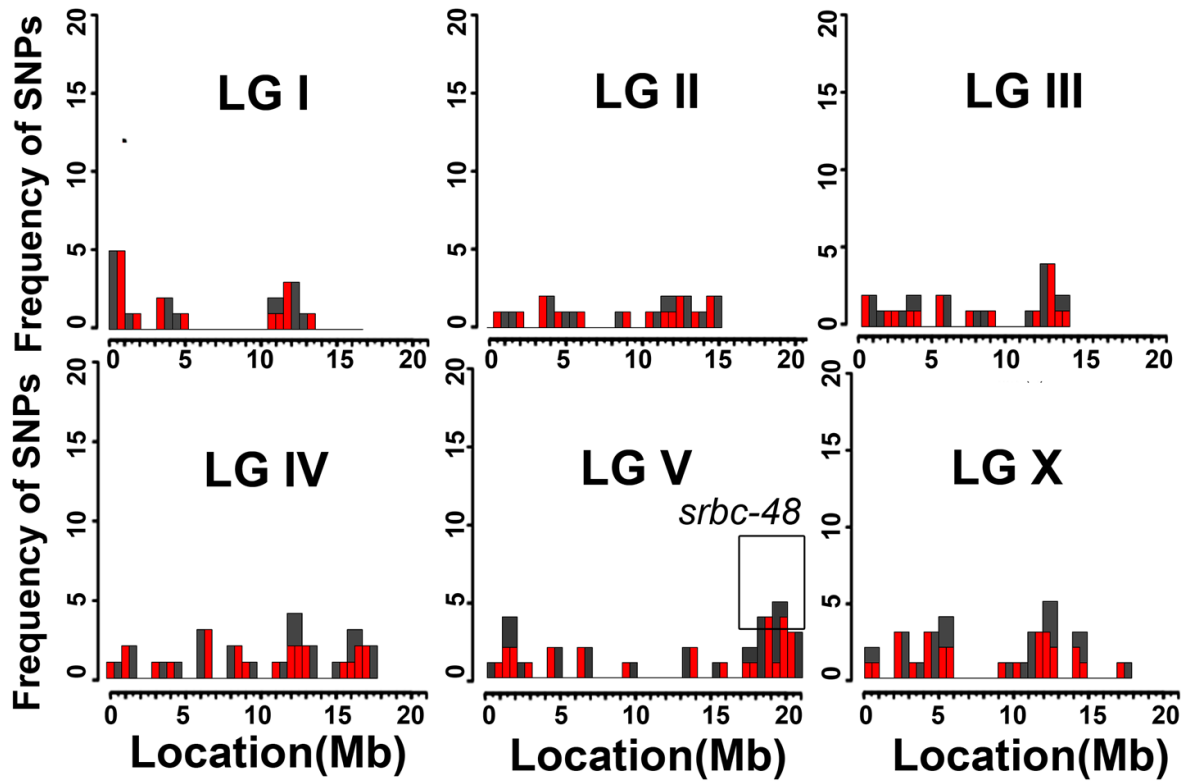
Figure S1. Linkage maps of single nucleotide polymorphisms (SNPs) for the mutant AY-23 showed the linkage in the V chromosome.
