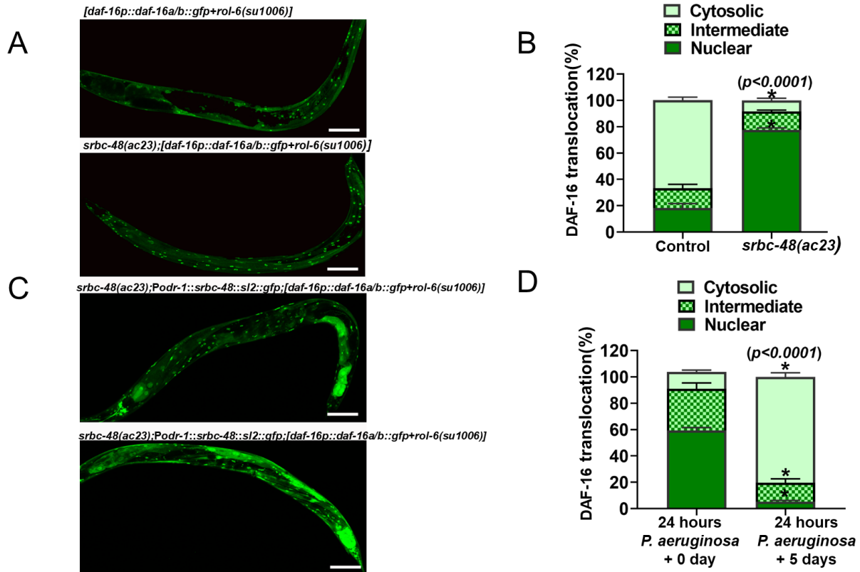
Figure S5. DAF-16 nuclear localization exhibited by srbc-48(ac23) animals is irreversible.
