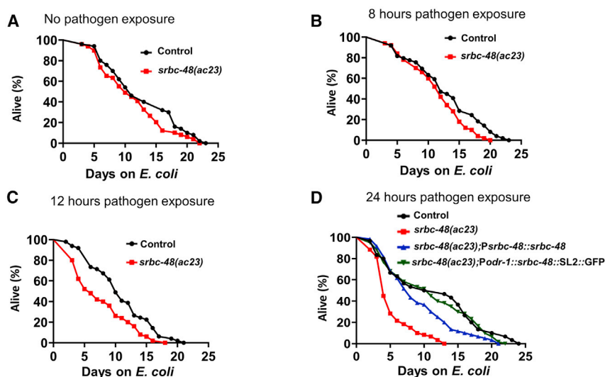
Figure 5. Pathogen Infection in srbc-48 Animals Results in a Reduced Lifespan
