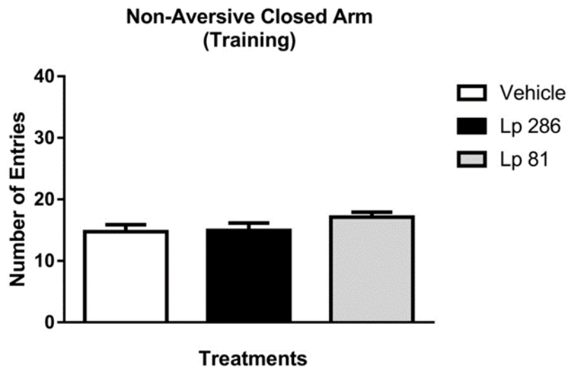
S2 Figure. Number of entries into the non-aversive closed arm of the apparatus during the training session of the plus maze - discriminative avoidance test. ANOVA: [F(2,45)=1.543; p=0.2249].
