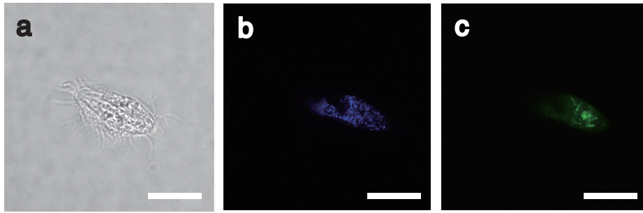
1 Supplementary Figure S1. Microscopic observations of Cyclidium sp. YH. a: Bright field. b: DAPI image. 2 c: Fluorescent micrograph after hybridization with archaea-specific probe (Arc915) for the endosymbiotic 3 methanogen of Cyclidium sp. YH. The scale bar represents 10 \mu m.
