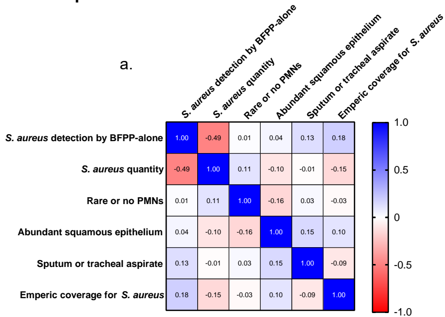
Figure S3. Pearson's correlation coefficient matrix for discordant detection of a) S. aureus and b) H. influenzae by BFPP compared to SOC
