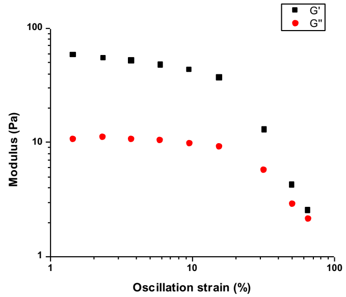
Supplemental Figure 2: Representative strain sweep (shown for RF crosslinking light dose of 0.5 \text{ J/cm}^2 at fixed frequency of = 20 \text{ rad/s} shows end of linear response (in this case around 10% strain) and material failure used to estimate yield stress.
