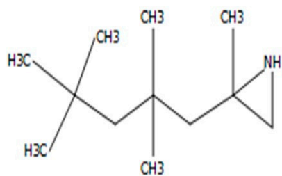
Aziridine, 2-methyl-2-(2,2,4,4-tetramethylpentyl)-
