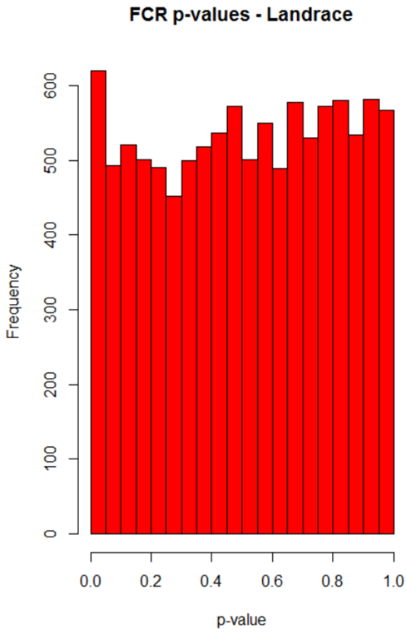
Supplementary figure 1 – Distribution of P-values in the Differential expression analysis for FCR in Danbred Landrace(left) and Danbred Duroc(right)
