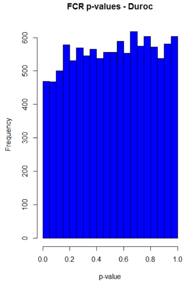
Supplementary figure 1 – Distribution of P-values in the Differential expression analysis for FCR in Danbred Landrace(left) and Danbred Duroc(right)
