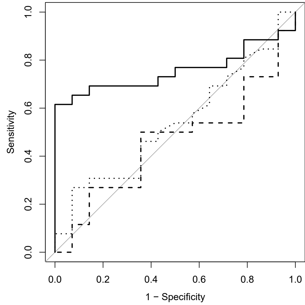
Plasma glucose
