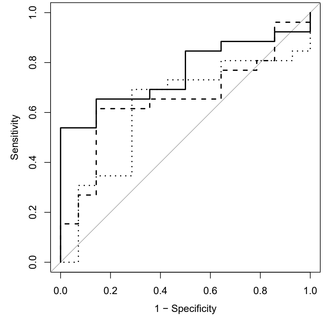
Urinary galactose/creatinine
