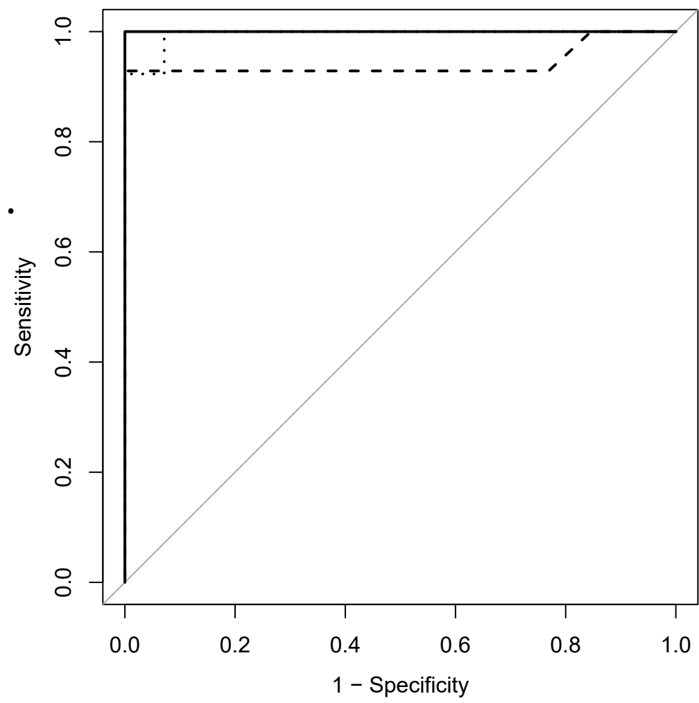
Breath H2
