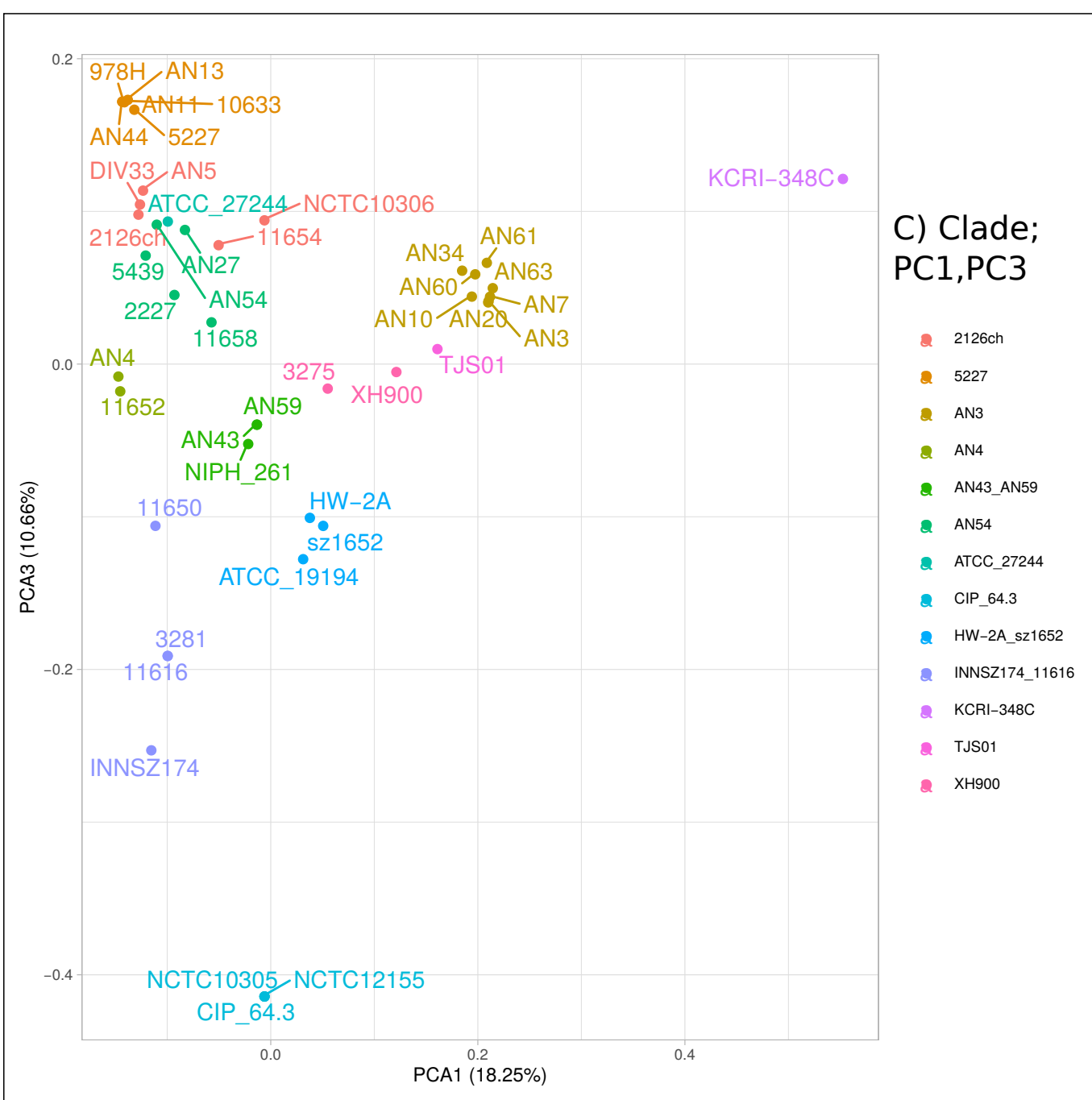
Supplementary Figure 5. Principal component analysis of the SNVs in the core genome.
