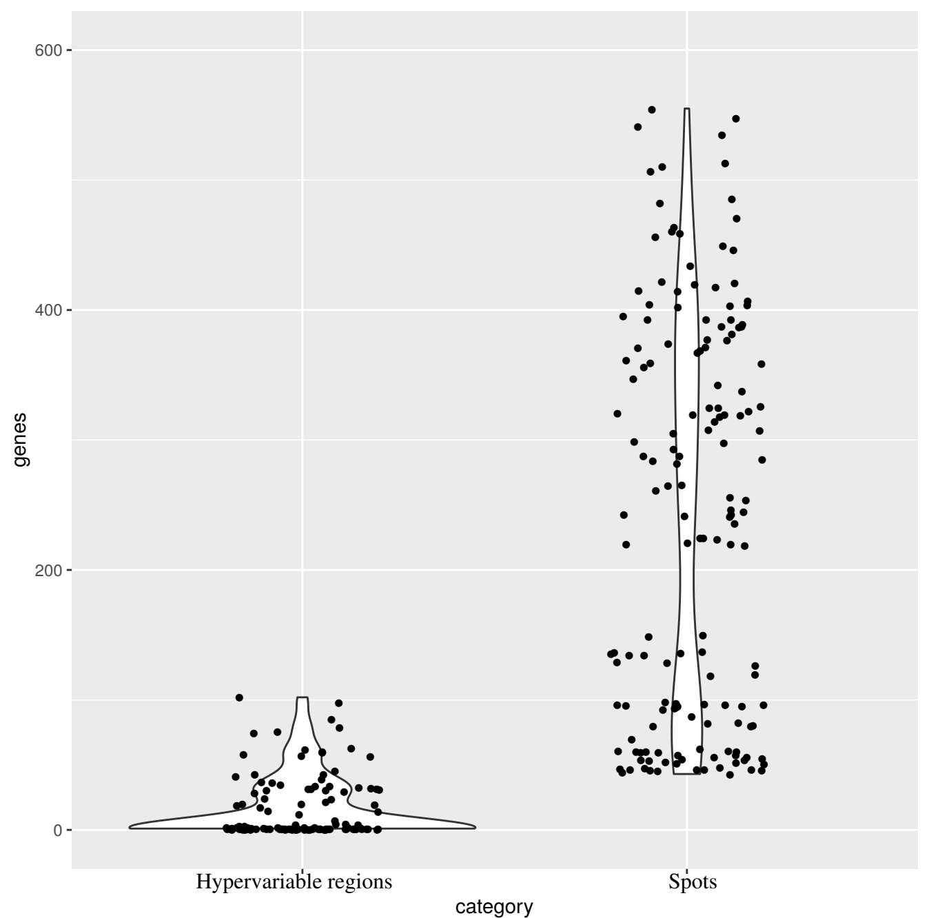
Supplementary Figure 6. Violin plot of the number of genes inside spots and hypervariable regions.
