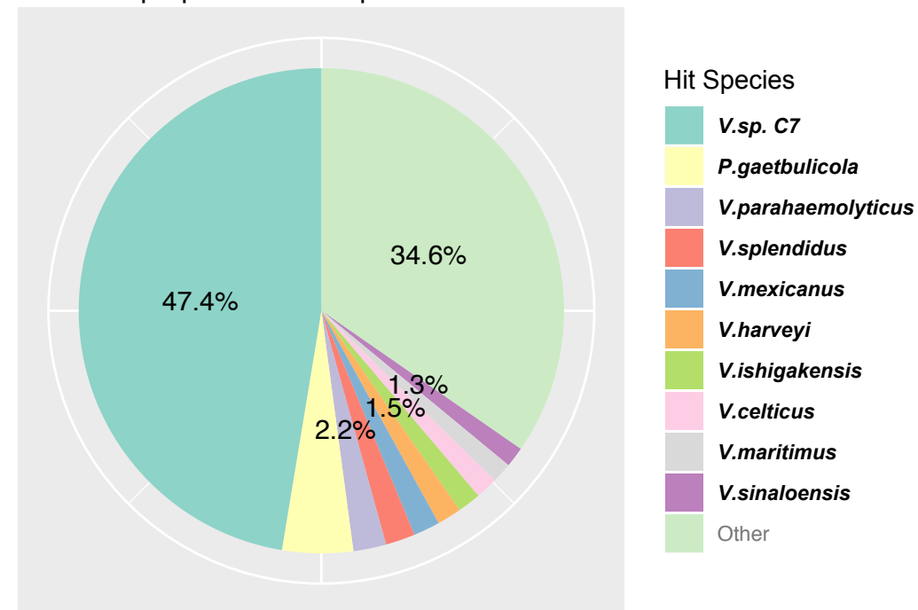
B The proportion of hit species for Vas2
