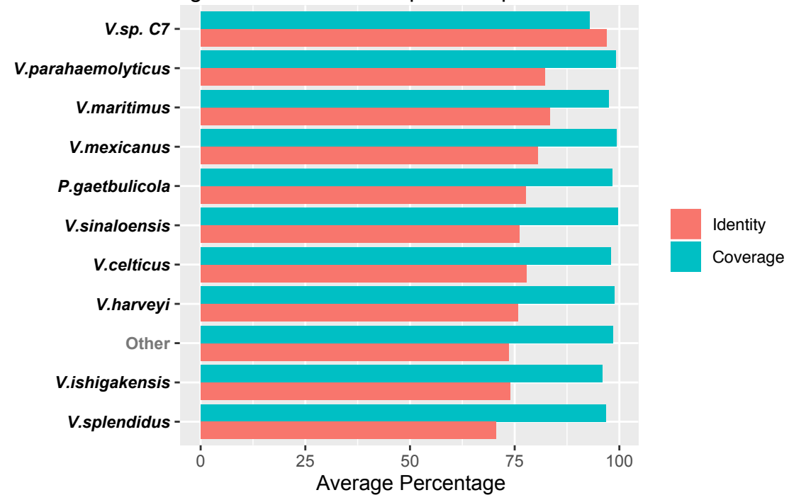
D Alignment statistics of top 10 hit species for Vas2
