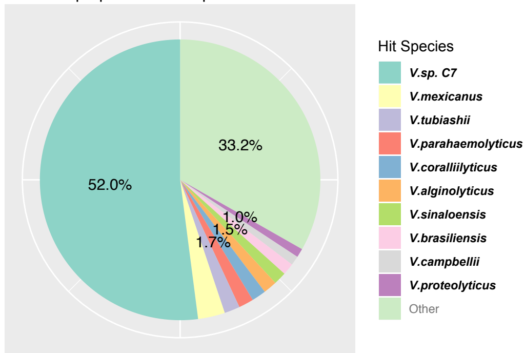
A The proportion of hit species for Vas1
