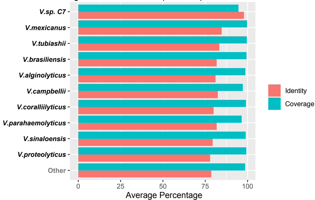
C Alignment statistics of top 10 hit species for Vas1
