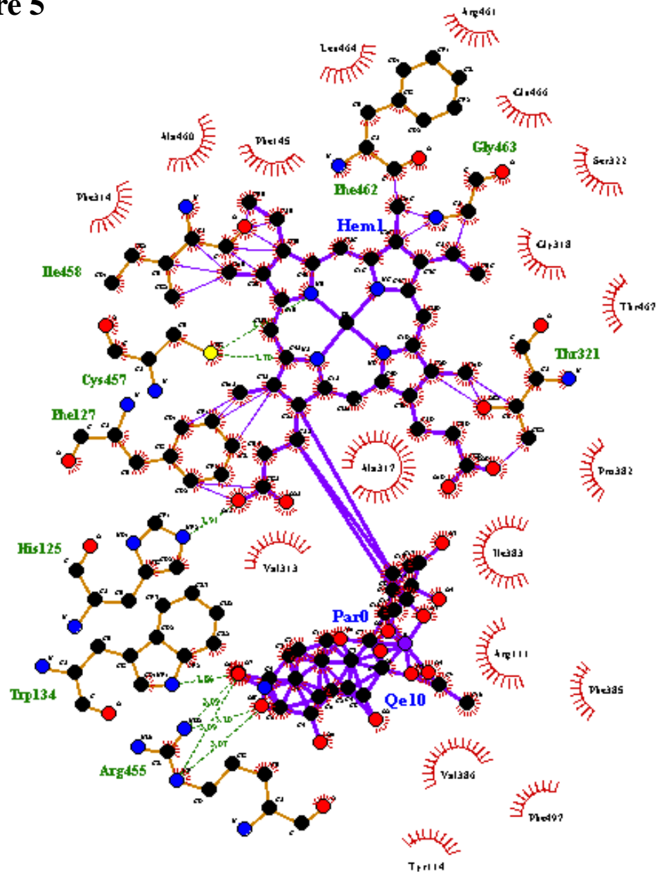
CYP6BK3_Heme_Model_Q1 TD Paraoxon
