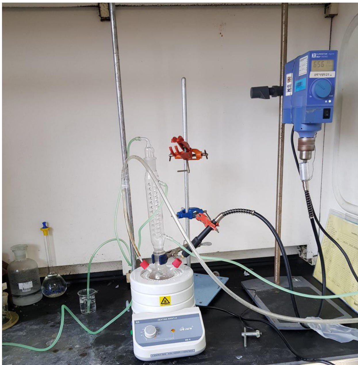
Supplementary Figure S1. These experimental setups and equipment were used to produce \text{Fe}_3\text{O}_4@\text{CA} nanoparticles.
