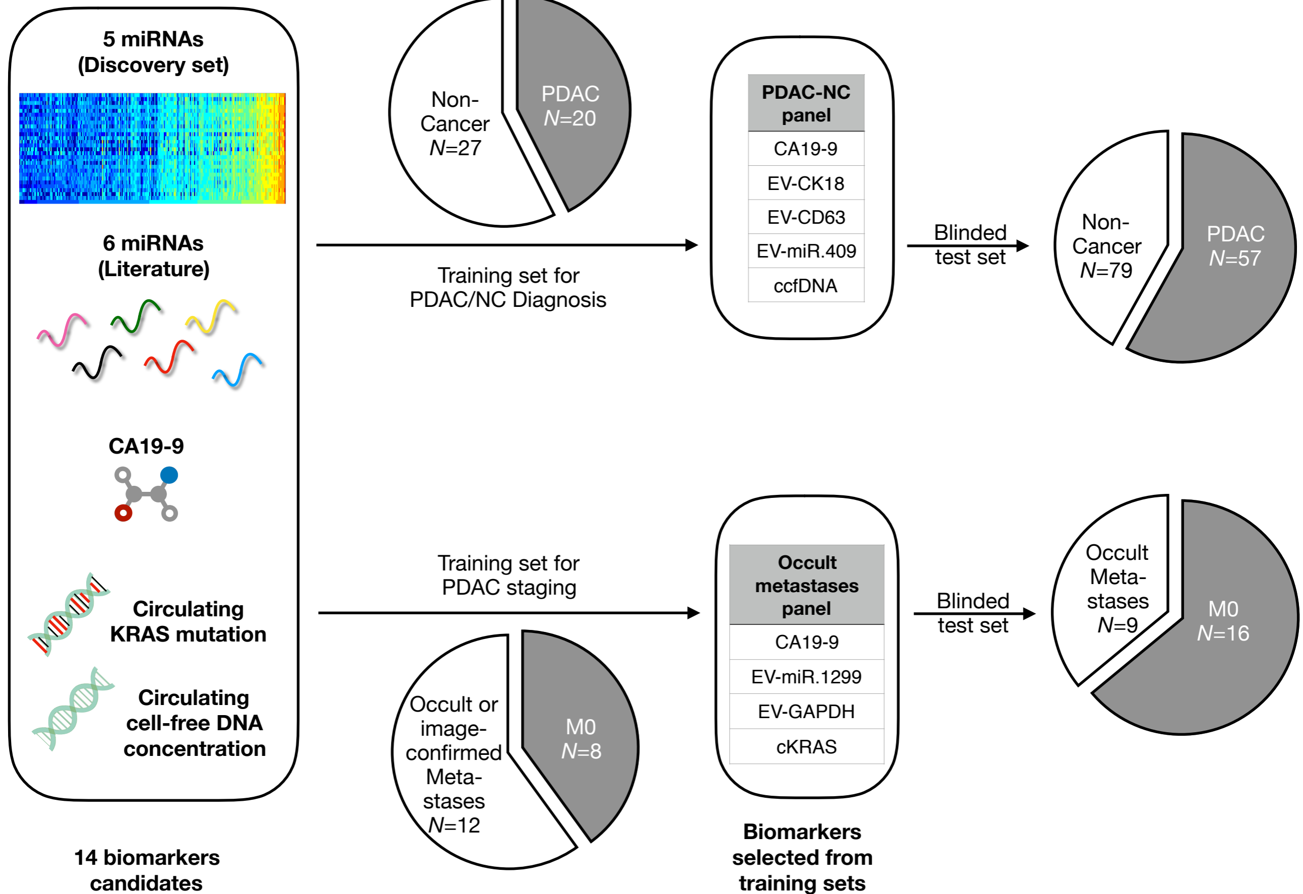
Figure S3. Multi-analyte panel generation procedure of PDAC/NC diagnosis and occult metastases detection
