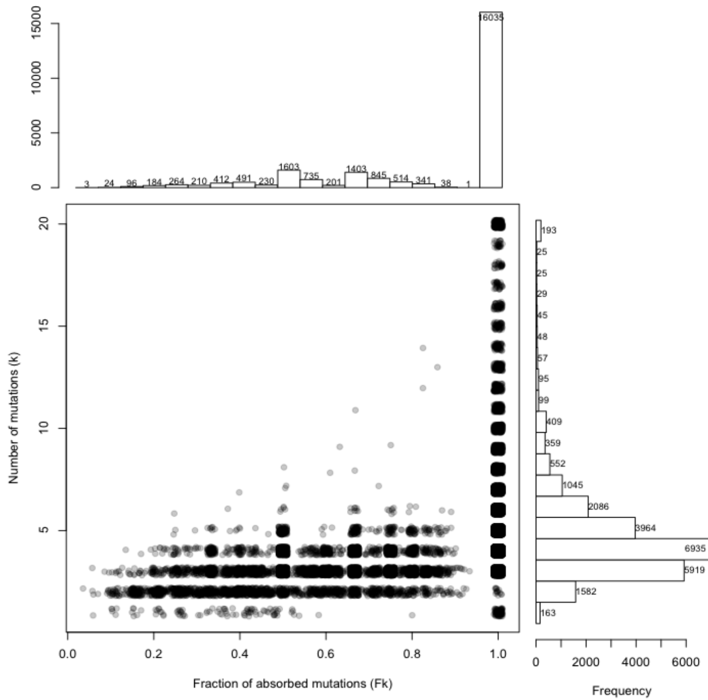
Fitted F_k values in TCGA data
