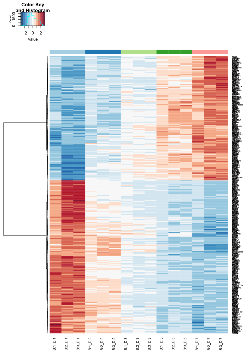
Genes with DE \leq 2 were selected to generate the multidimensional scaling (MDS) plot (A) and heatmap (B) to show the effect of the batch adjustment and monotonic gene expression patterns across the samples at different days respectively.
