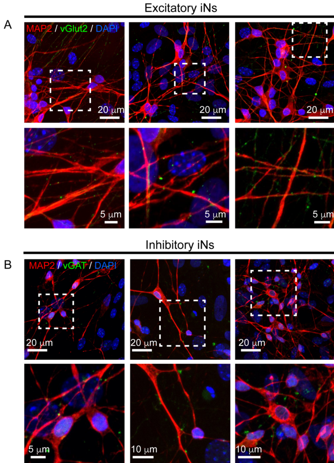
Figure S2. Morphological characterization of excitatory and inhibitory neurons. Both neuronal subtypes were grown on glass coverslips and imaged at 63X. A) Excitatory iNs show presence of both MAP2 and vGlut2 suggesting an excitatory phenotype. B) Inhibitory iNs are positive for MAP2 and vGAT, suggesting an inhibitory phenotype. Dashed white boxes correspond to zoomed in area shown below each image.
