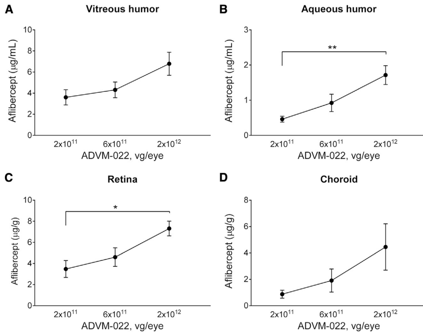
Figure 2. Aflibercept Expression Levels as a Function of ADVM-022 Dose in vitreous humor (A), aqueous humor (B), retina (C) and choroid (D), collected at Day 56 Post-dose (n = 4 Eyes/2 Animals) Means \pm SEM for treatment groups are shown. *p < 0.05, **p < 0.01 (one-way ANOVA with Tukey's multiple comparisons test).
