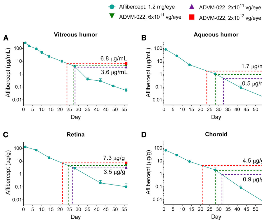
Figure 1. IVT ADVM-022 Provides Levels of Intraocular Aflibercept Expression Comparable with Those Measured 21–32 Days following IVT Injection of Aflibercept Recombinant Protein (n = 4 Eyes, 2 Animals for Each Data Point)
