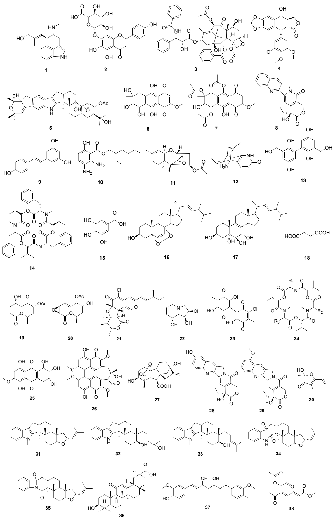
Figure S1. Structures of the secondary metabolites listed in Table 1 and 2
