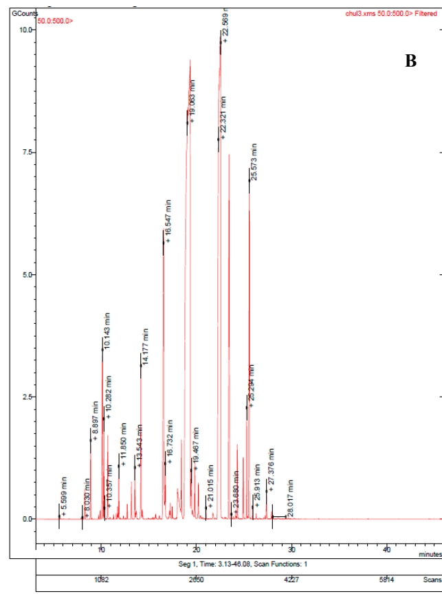
Supplementary Figure 1. GC-MS chromatograms of essential oils from three Korean native Thymus quinquecostatus cultivars. A, Odae cultivar; B, Wolchul cultivar; C, Jiri cultivar.
