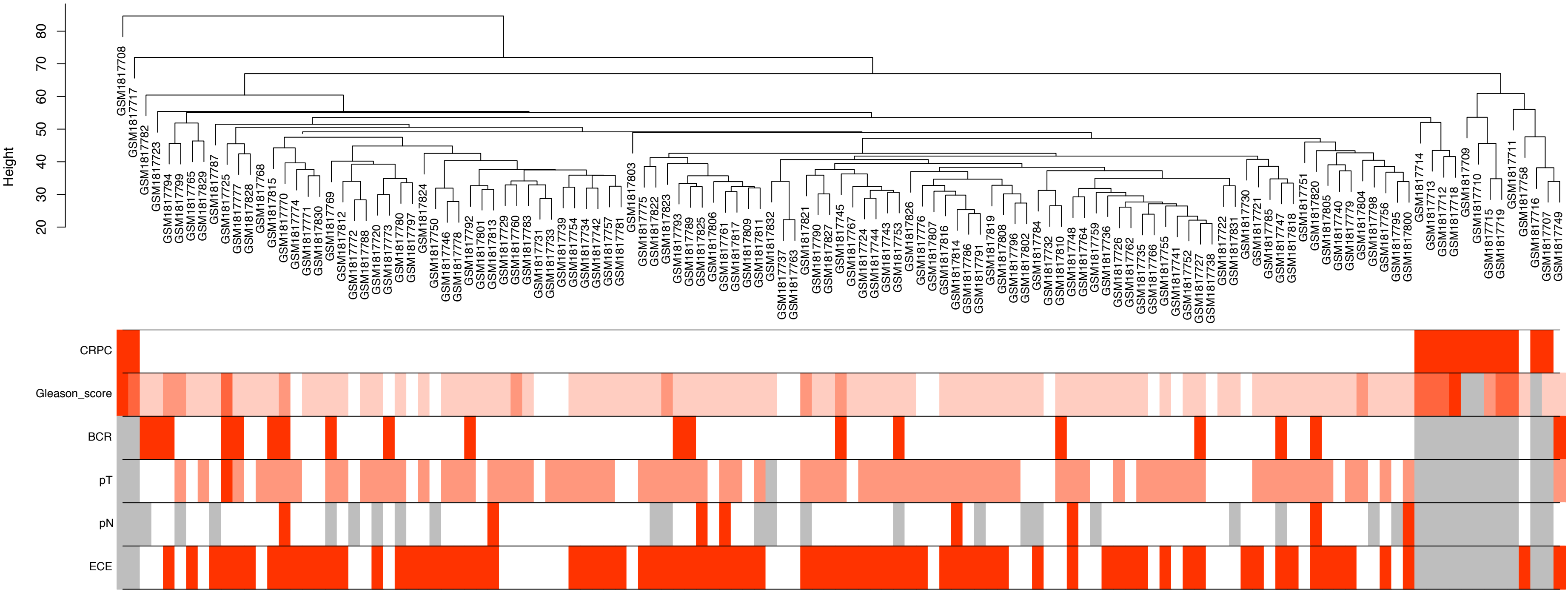
Sample dendrogram and trait heatmap
