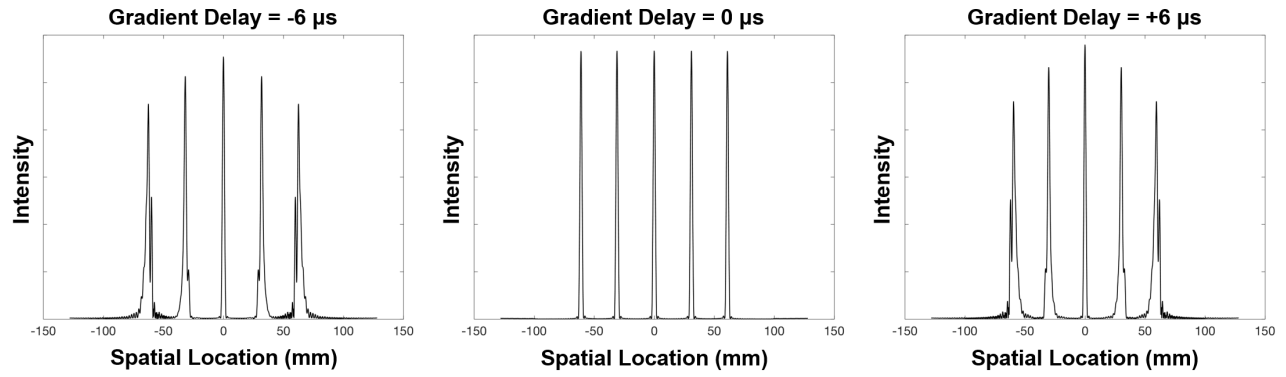
Supporting Information Figure S1. Point-spread-functions as a function of distance from FOV center at gradient delays of -6, 0, and +6 \mu\text{s} . The locations of these point objects were matched to those of the five small samples shown in Figure 3 .
