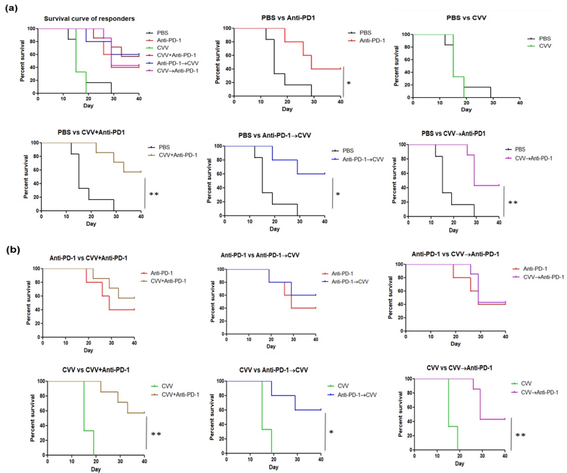
Figure S1. Survival curve analyses. Kaplan–Meier curves were plotted on the basis of tumor volume. Tumor volume >1000 \text{ mm}^3 was considered death. (a) Survival curve among responders. (b) Survival curve among responders: monotherapy vs. combination therapy. * p < 0.05 ; ** p < 0.01 .
