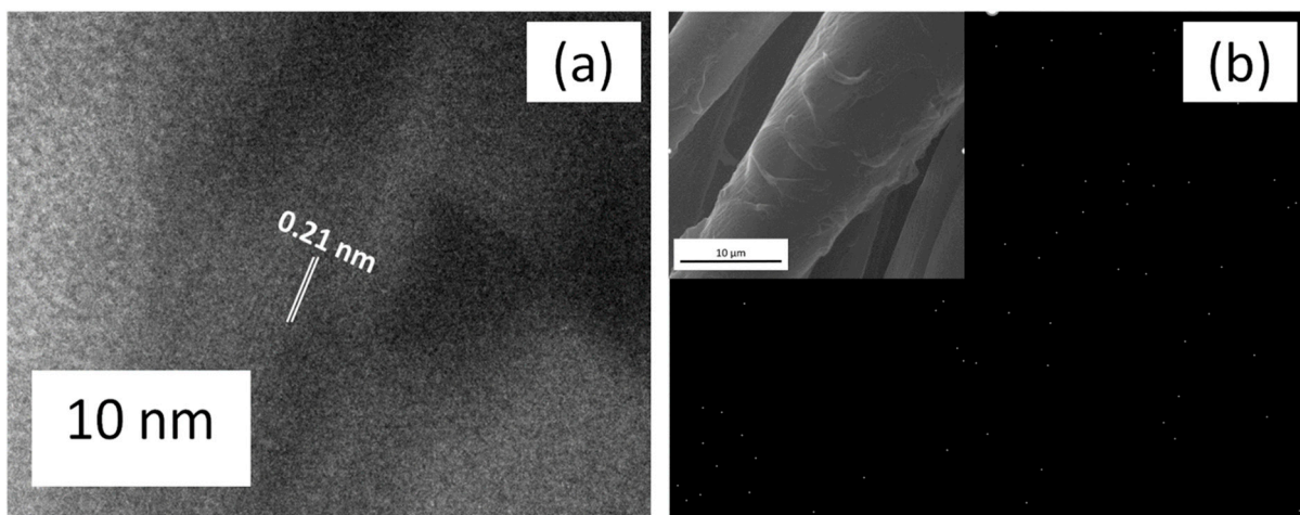
Figure S1. (a) HRTEM image of CuNWs, and (b) EDX mapping of the CuNWs/CC sample containing 0.1 pg CuNWs.
