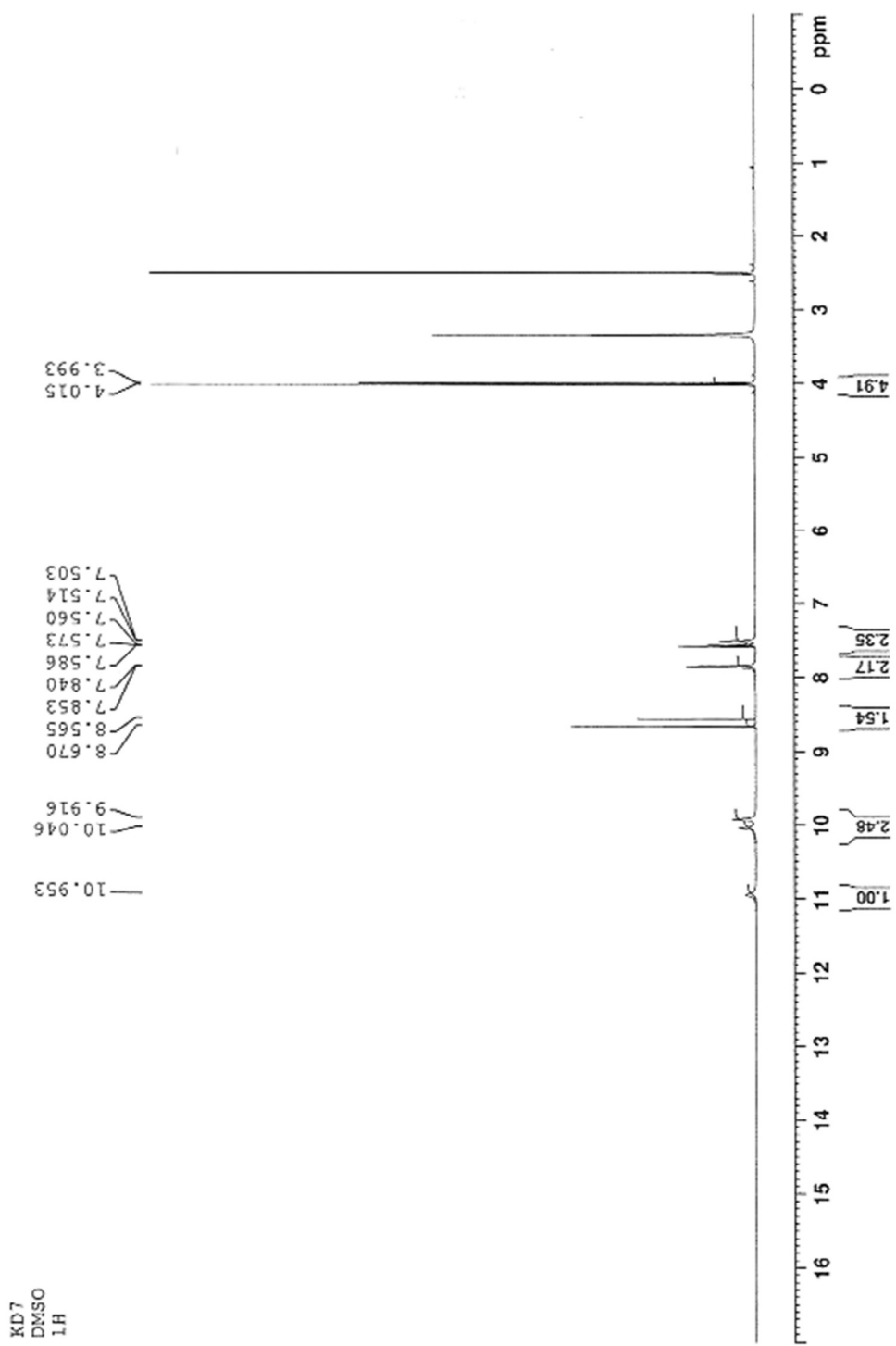
Compound 12.
