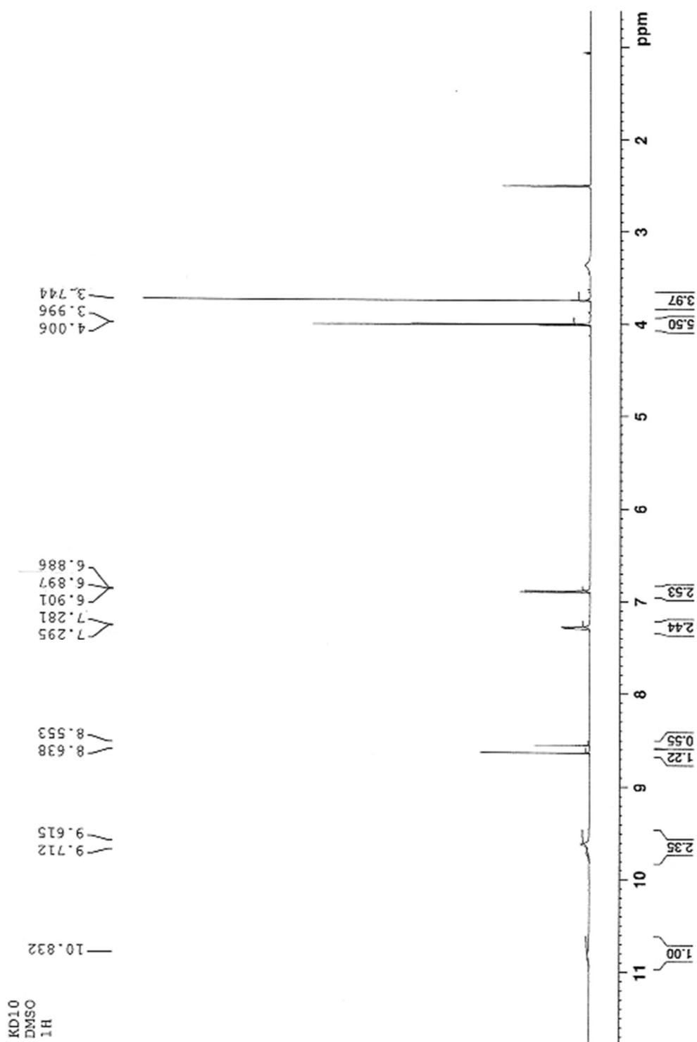
Compound 10.
