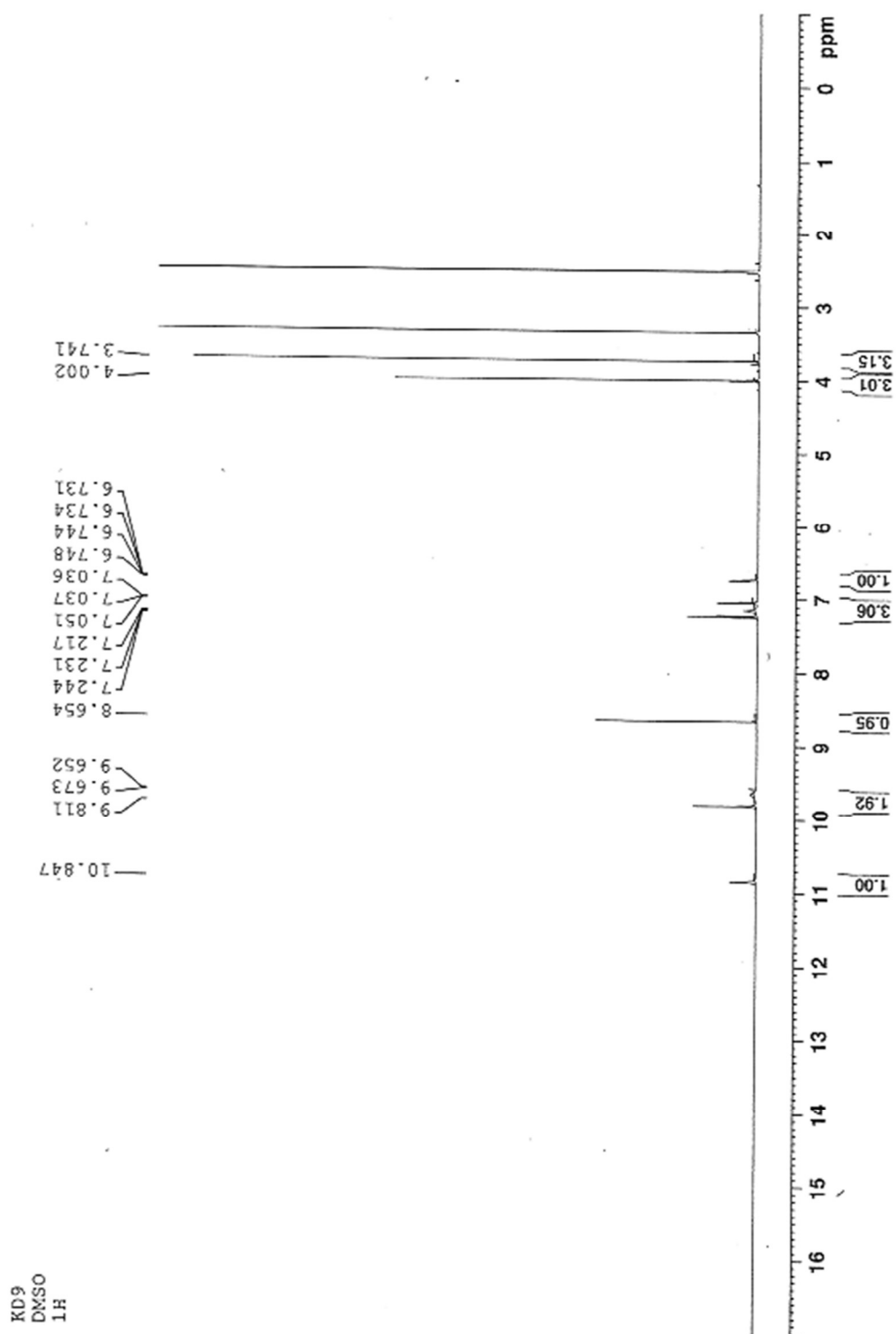
Compound 9.
