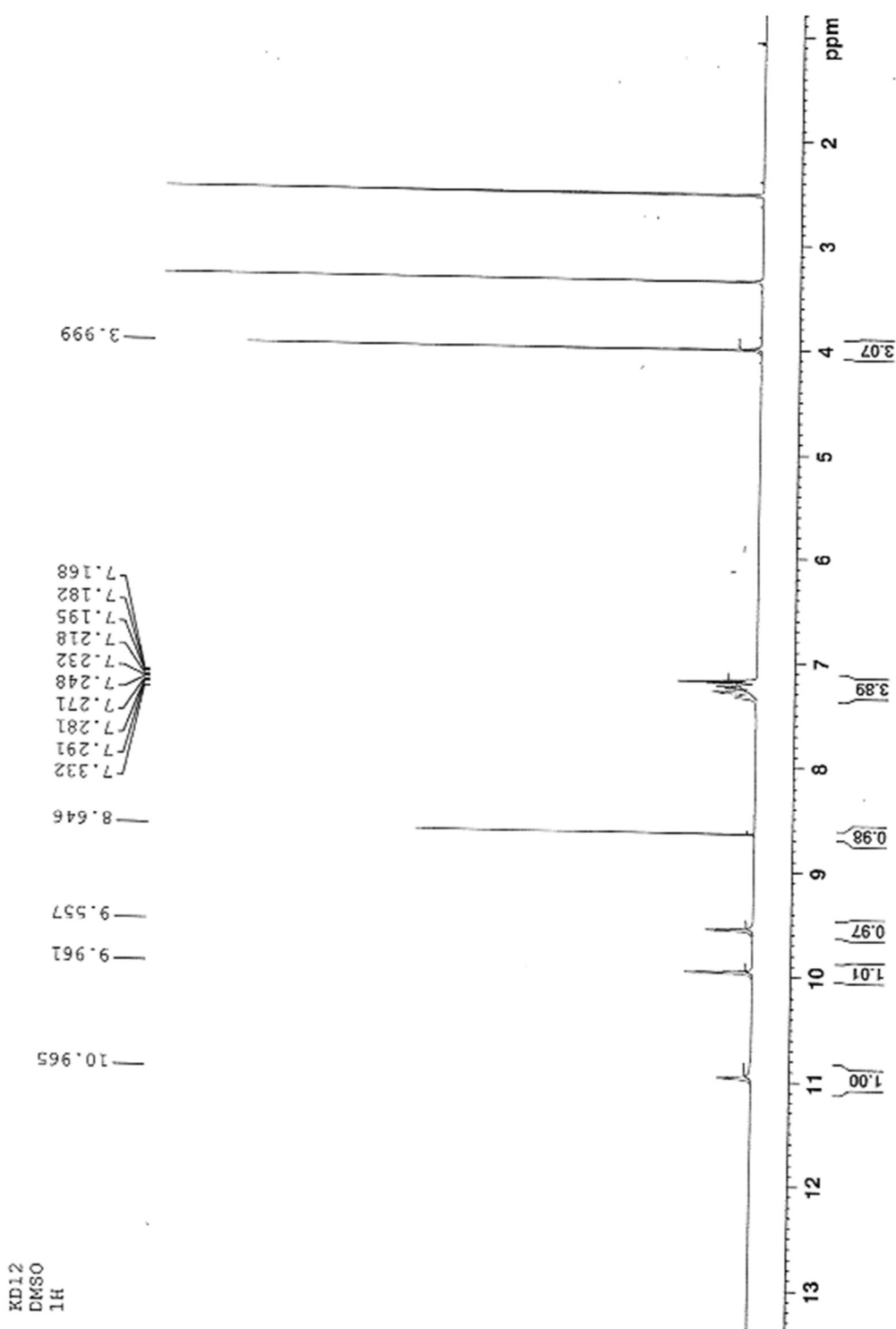
Compound 5.
