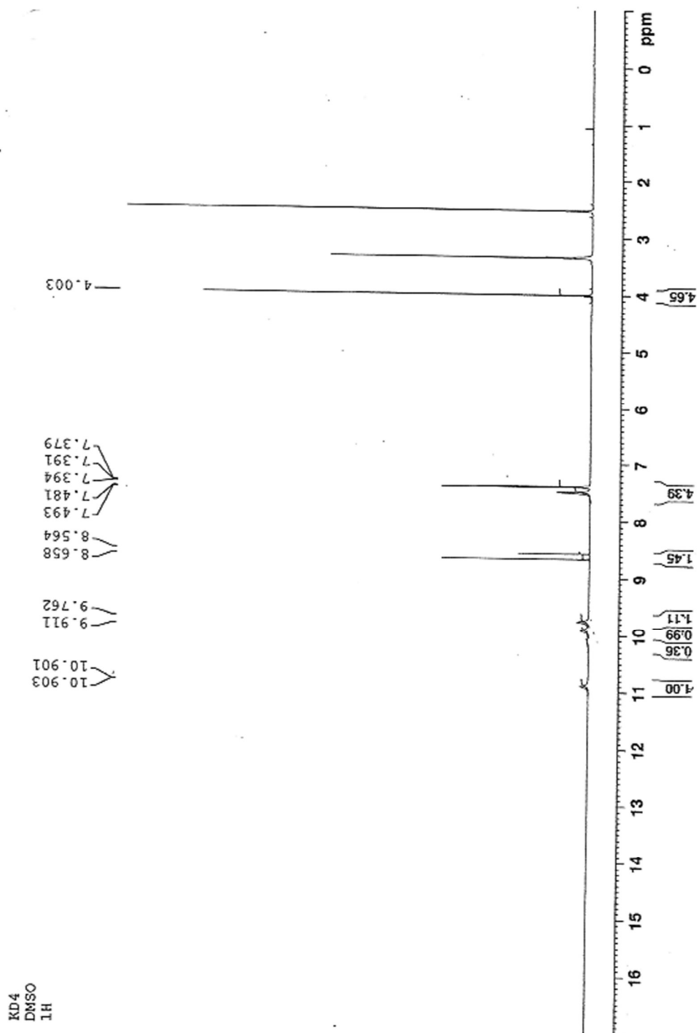
Compound 4.
