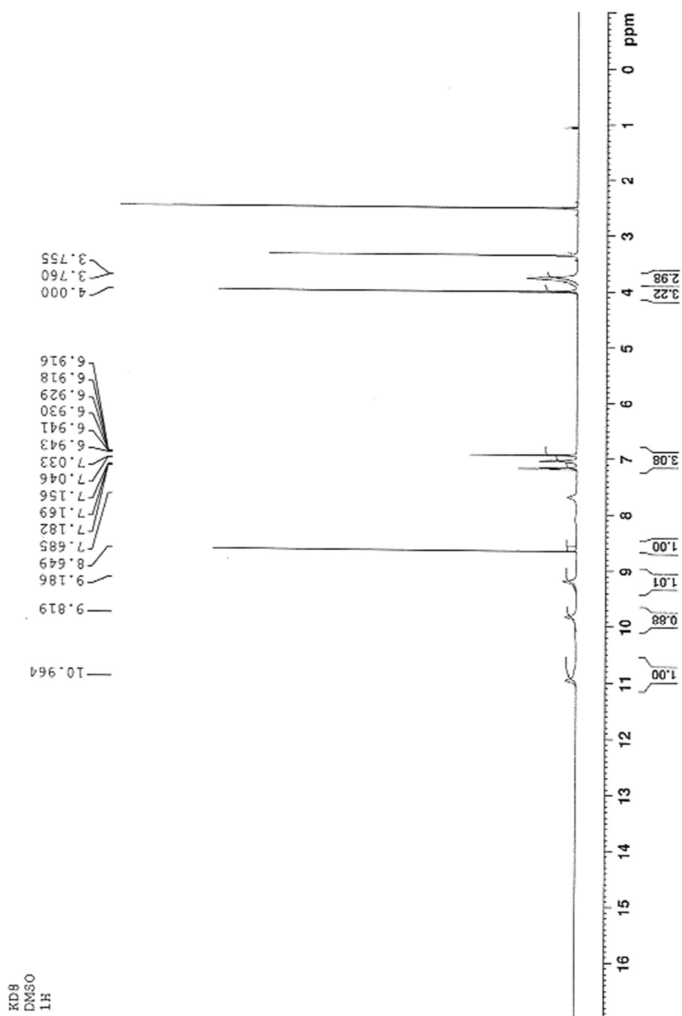
Compound 8.
