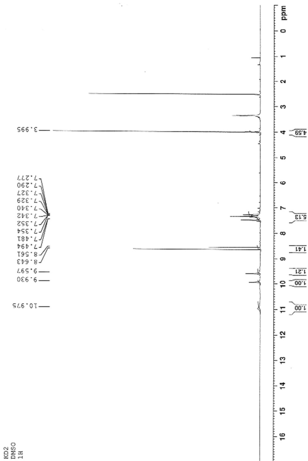
Compound 2.
