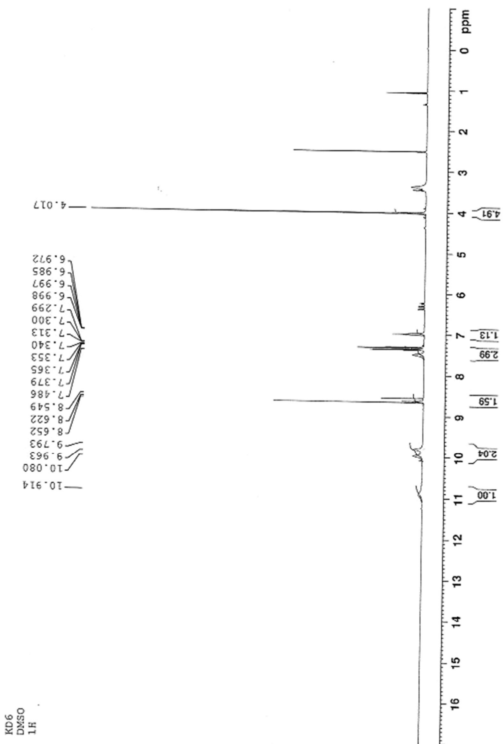
Compound 6.
