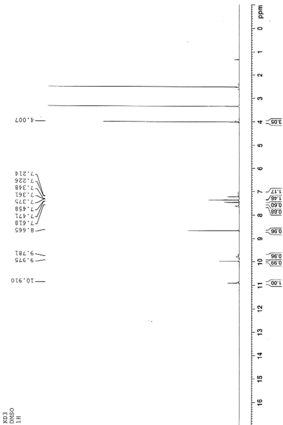
Compound 3.
