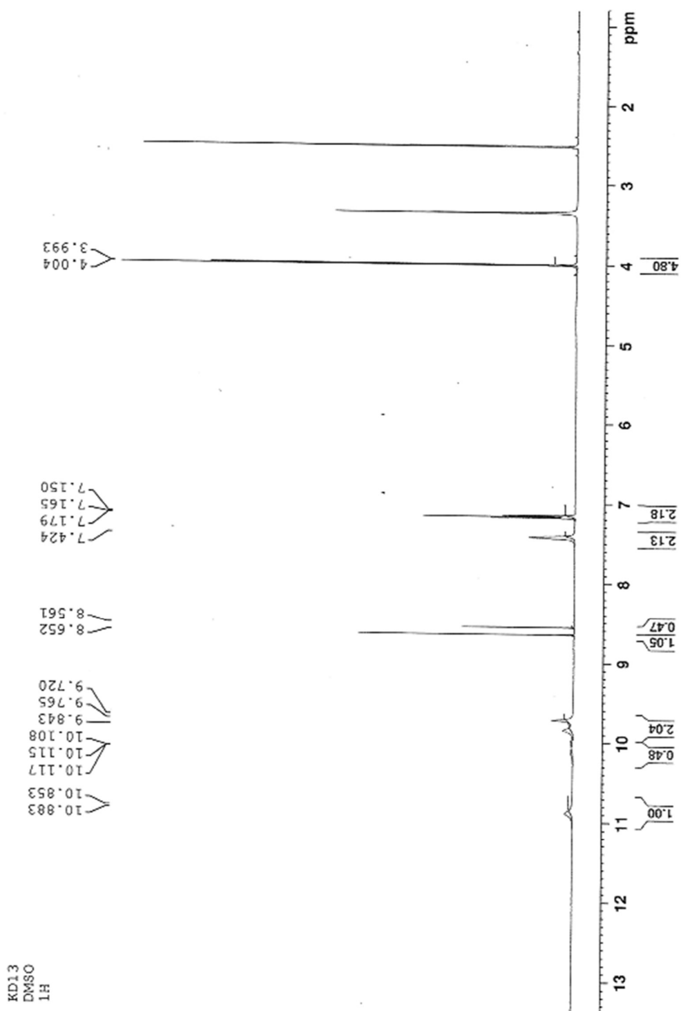
Compound 7.
