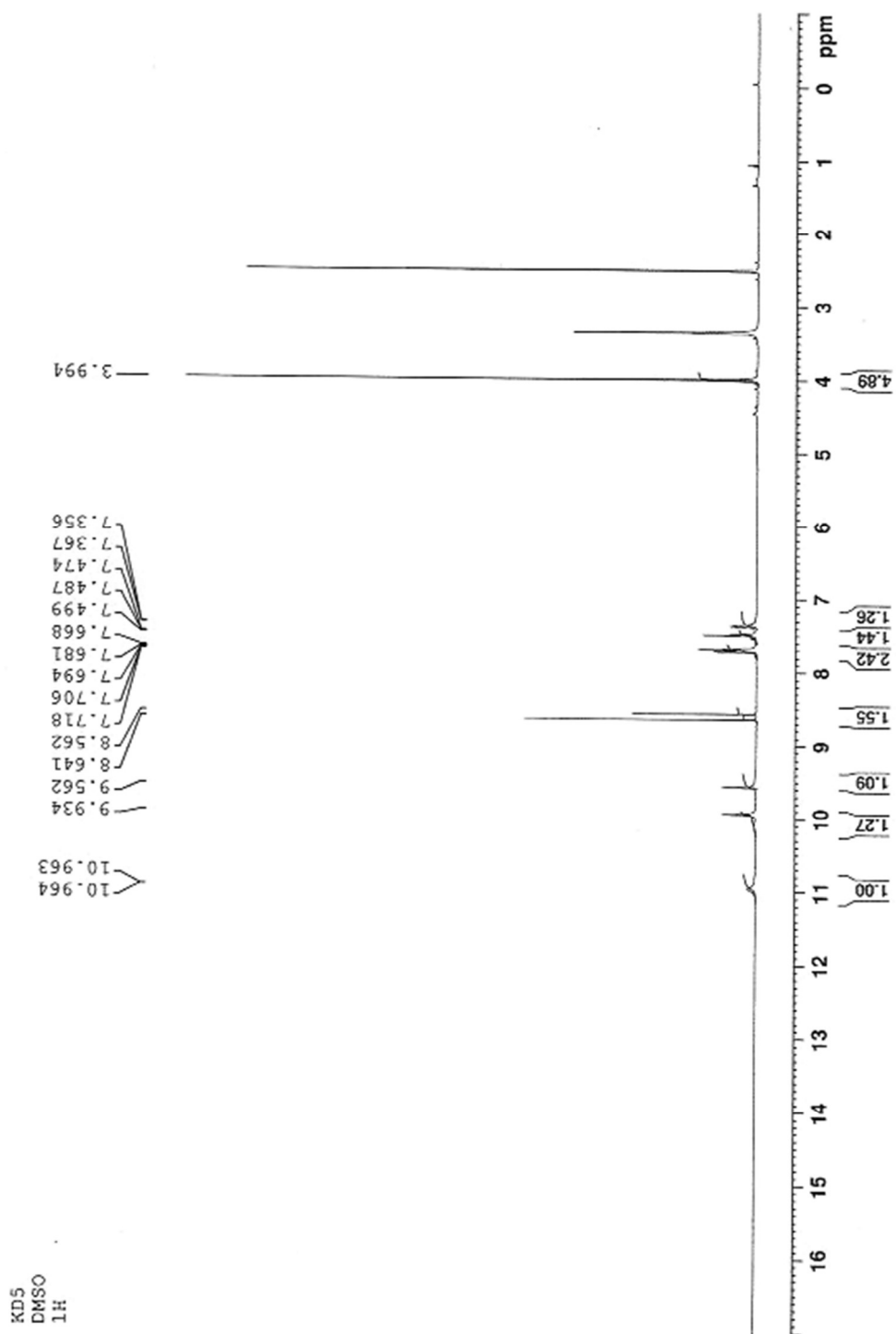
Compound 11.
