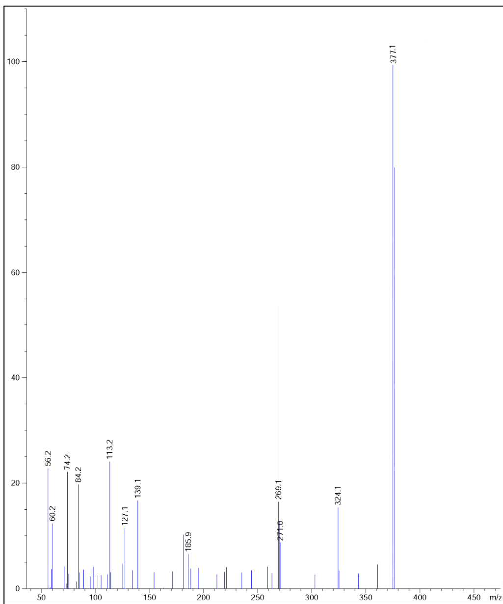
Figure S3: Mass spectrum of PIB ligand.
