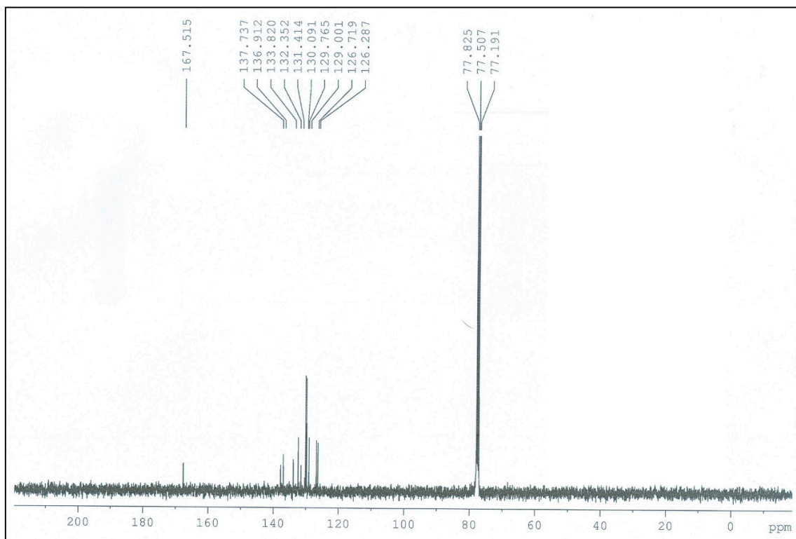
Figure S5: ^{13}\text{C} -NMR spectrum of PTM ligand.
