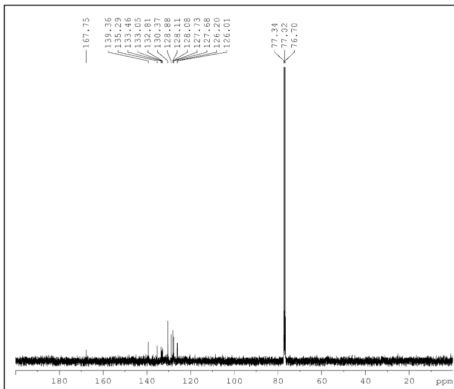
Figure S2: ^{13}\text{C} -NMR spectrum of PIB ligand.
