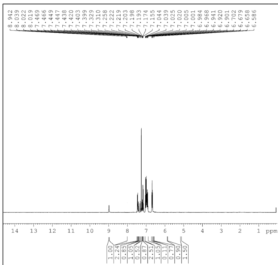
Figure S1: 1 H-NMR spectrum of PIB ligand.
