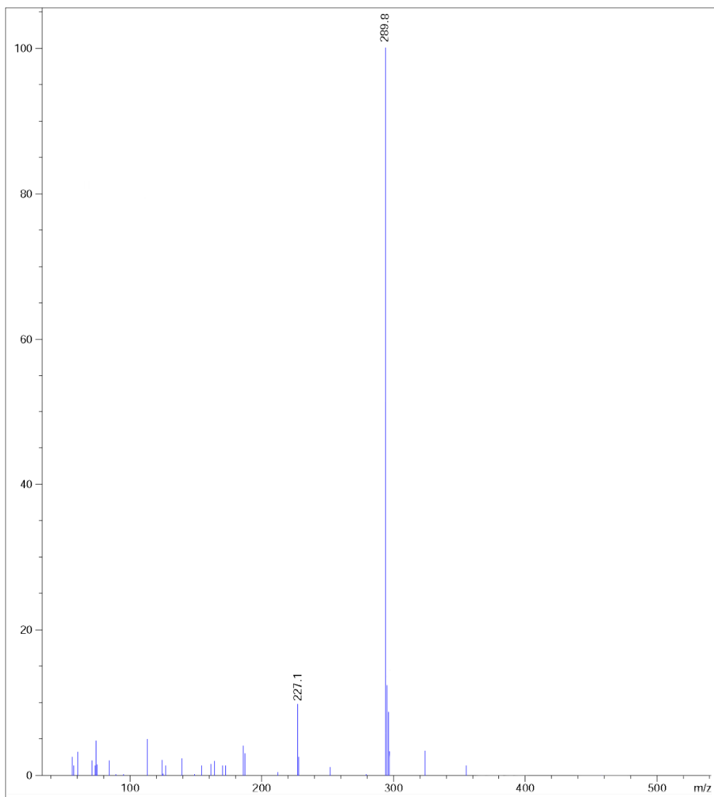
Figure S6: Mass spectrum of PTM ligand.
