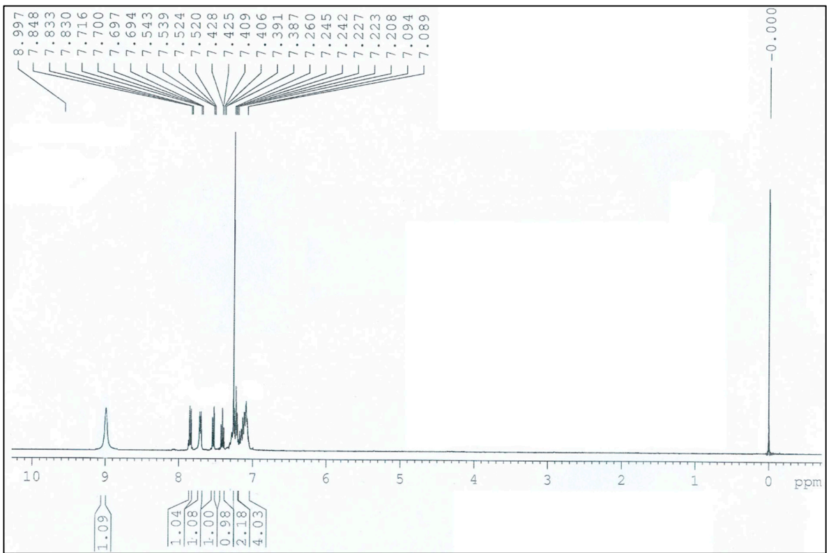
Figure S4: 1 H-NMR spectrum of PIB ligand.
