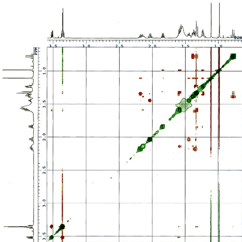
NOESY spectrum
