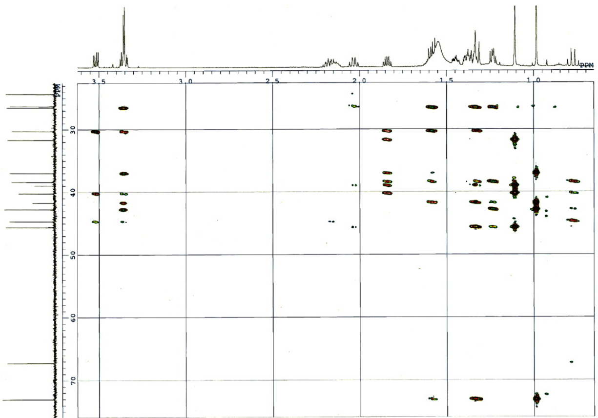
HMBC spectrum
