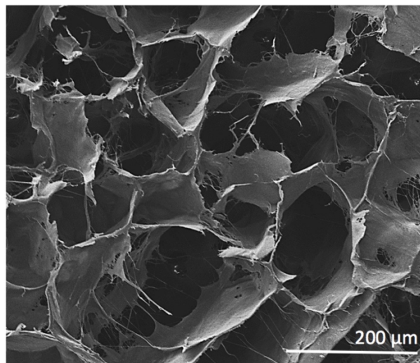
Supplementary Figure 1. Scaffold structure characterization by SEM of Coll.
