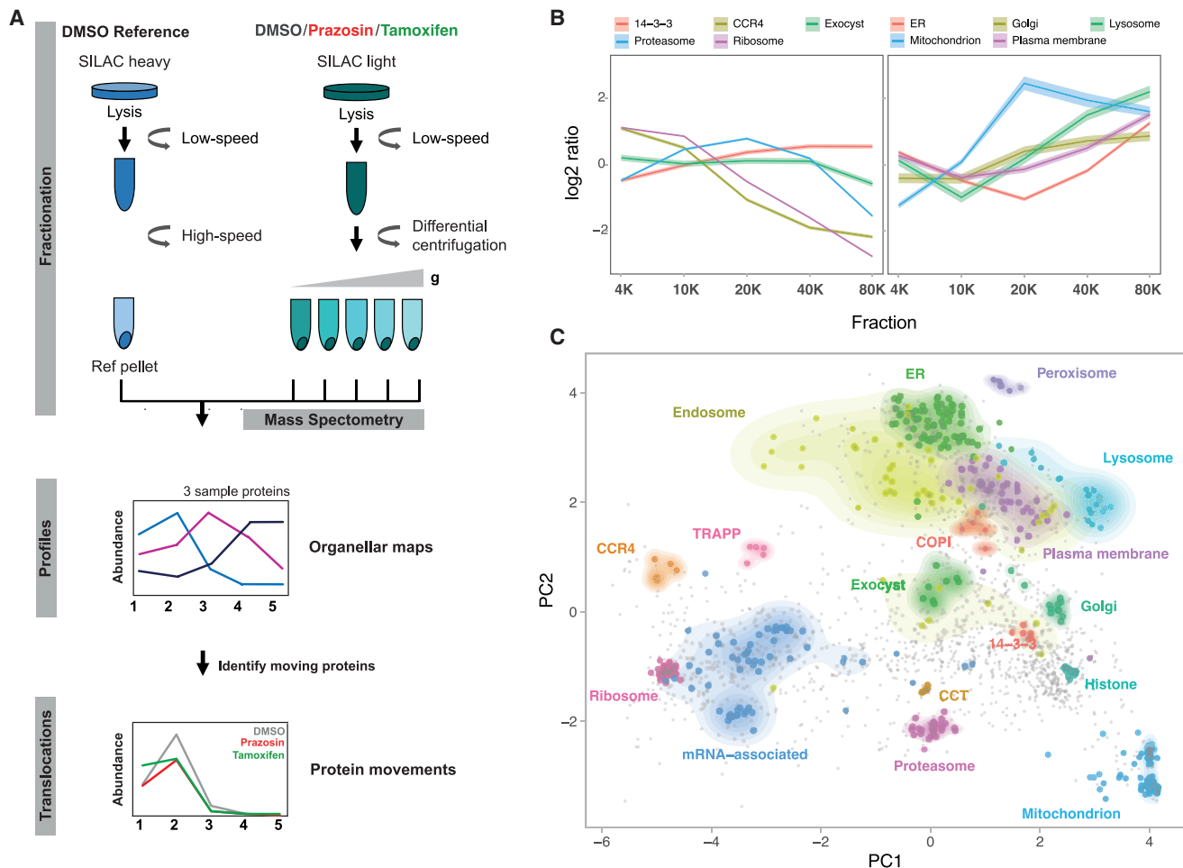
Figure 2. Organellar Mapping in Dendritic Cells
