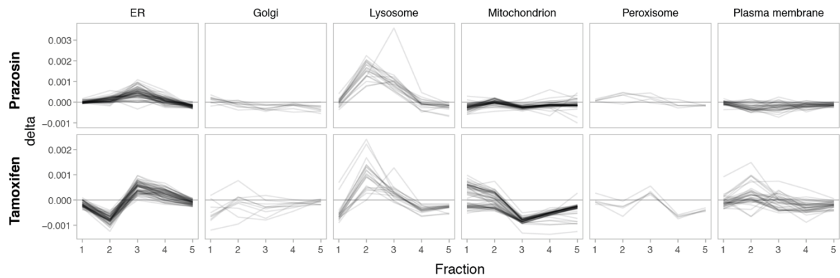
Figure S3. ‘Movement’ data for proteins from selected organelles used for ‘MR’ analysis.
