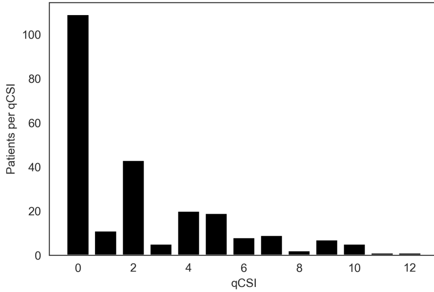
Figure S2: Frequency plot of validation cohort qCSI.
