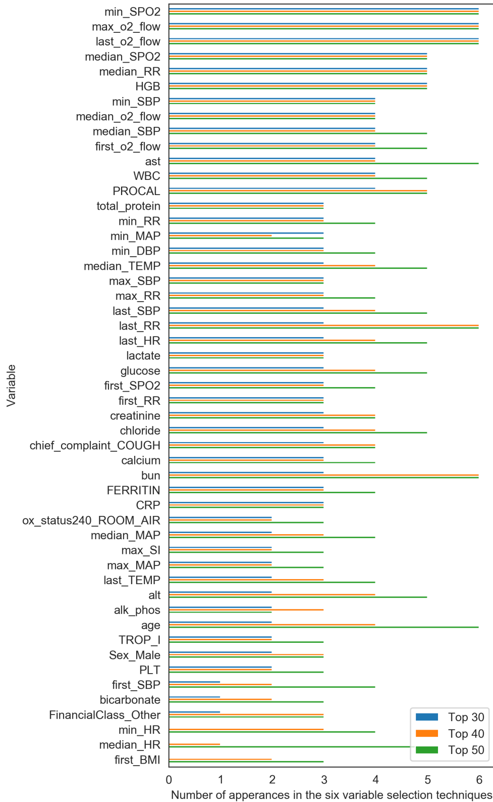
Figure S1: Six variable selection methods were used to identify potentially predictive variables. We limited each technique to the top 30, 40, and 50 variables of each of the methods and counted the number of models that each variable was identified by. Here, we show only those features identified by three or more models.
