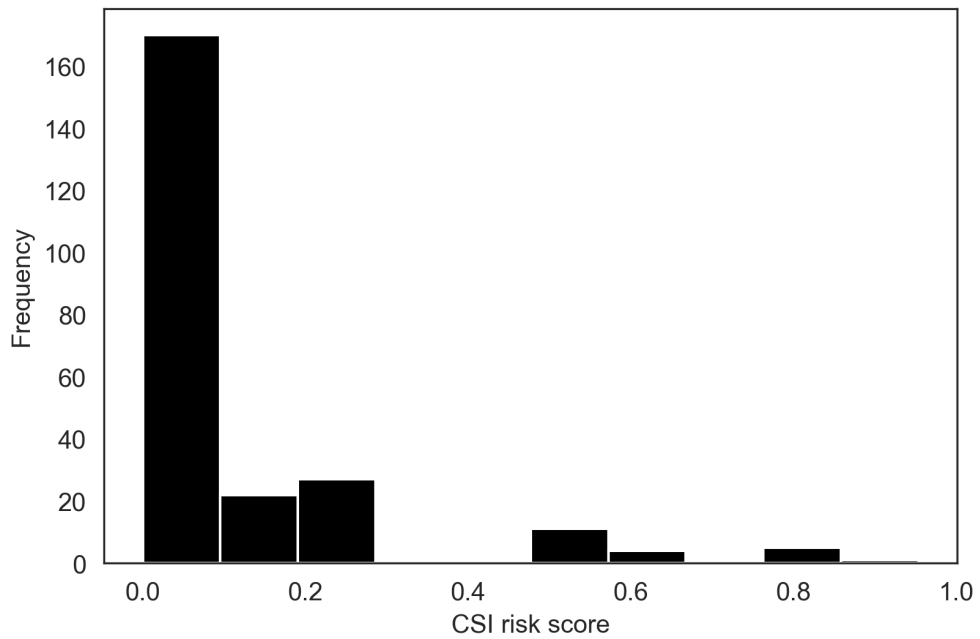
Figure S3: Frequency plot of validation cohort CSI. The CSI was generated by first training the gradient boosting model on the training cohort with cross-validation and isotonic regression. The best model was then retrained on the combined training and cross-validation cohorts. This model was then used to assign CSI to the external validation cohort.
