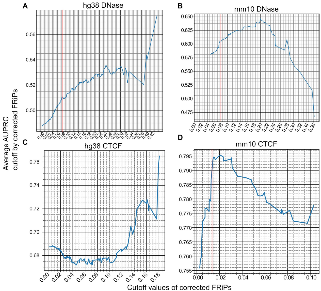
S4 Fig. The average of AUPRCs with various cutoff values of corrected FRiP. (A, B) Plots of average AUPRCs for human and mouse DNase-seq data (A and B) and CTCF data (C and D) as a function of cutoff values of corrected FRiPs. Note that increase in cutoff values of the corrected FRiPs results in an increase of the average AUPRCs, at least to some extent, except as shown in c. Red line, cutoff values for the filtered data in Fig. 2A and B.
