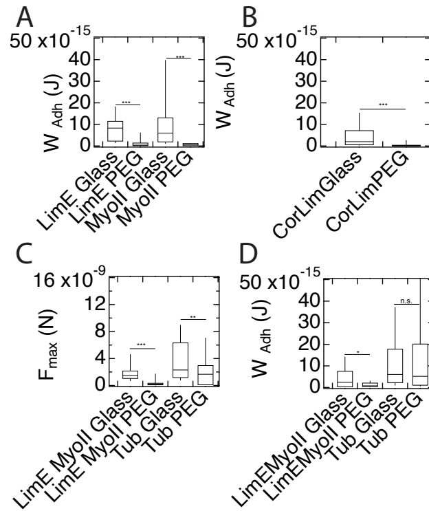
S7 Fig. Additional SCFS data: W_{adh} for developed AX2 cells expressing LimE-GFP or myoII-GFP (A) and for developed AX4 cells expressing LimE-GFP/corA-RFP (B). F_{max} for developed AX2 cells expressing both LimE-RFP and myoII-GFP, and alpha-tubulin-GFP (C) and the corresponding W_{adh} (D).
