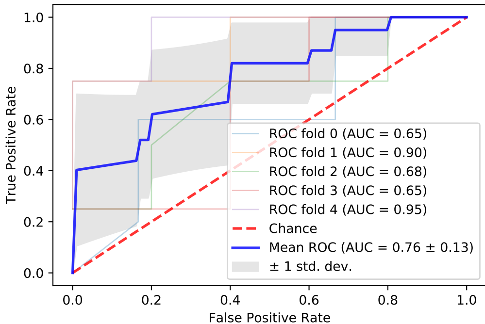
Receiver operating characteristic of selected genus
