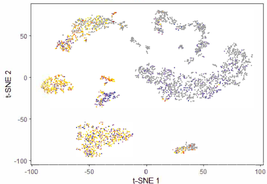
FOXJ1 Counts
