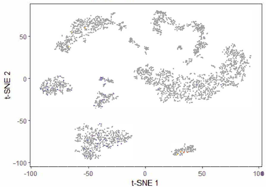
IL5RA Counts
