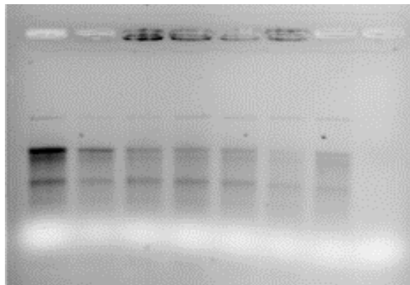
rsbW-sigF
