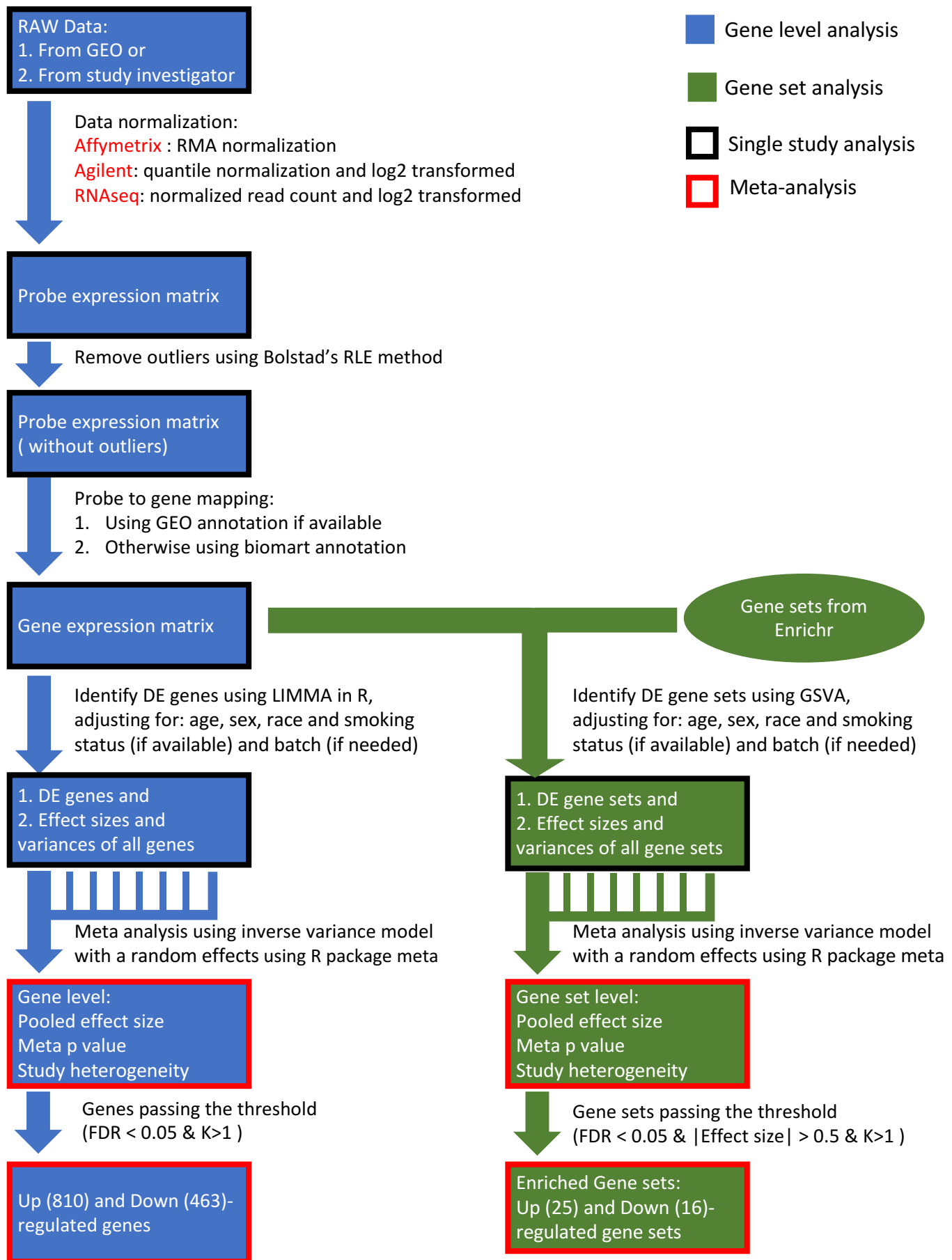
Supplementary Figure 1. Flowchart of workflow from data acquisition through meta-analysis.
