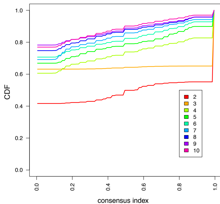
consensus CDF
