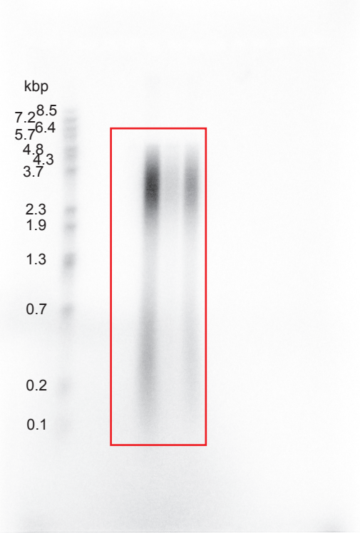
Figure 5A Autoradiograph
