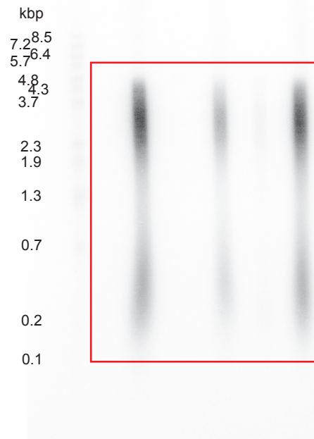
Figure 6B Autoradiograph
