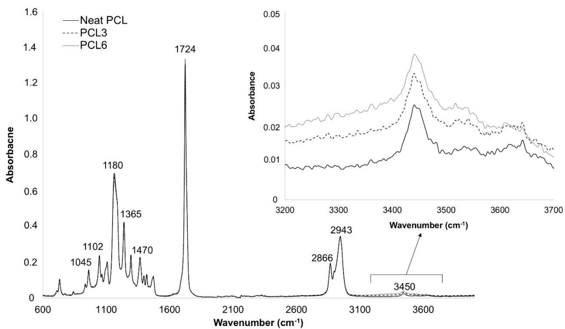
Figure S2: ATR-FTIR analysis of PCL and PCL/ASE composite films,
