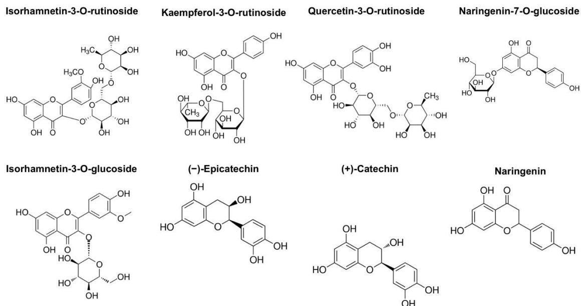
Figure S1: Chemical structure of main polyphenolic composition of ASE,
