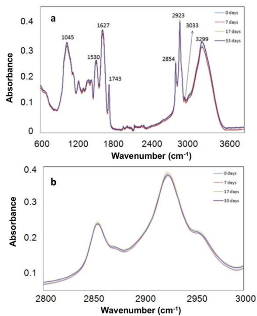
Figure S4: ATR-FTIR analysis of fried packaged almonds in PCL and PCL/ASE composite films with storage time.
