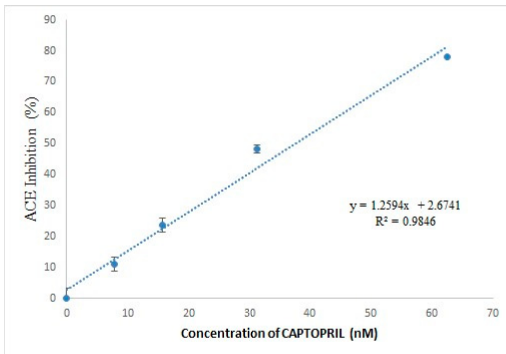
Figure S1. Standard curve of ACE inhibition using Captopril.
