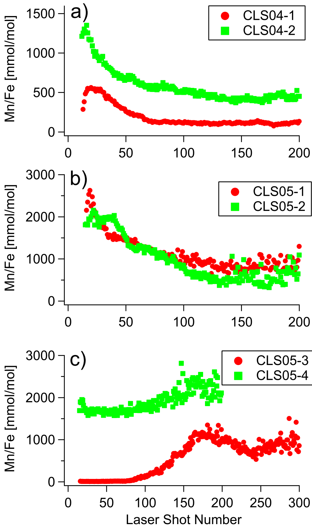
S4 Figure. fs-LA-ICPMS spot measurement profiles on rock varnish samples. The x-axis represents successive laser shots on the same spot. Each laser shot corresponds to a depth increment of about 50-100 nm.
