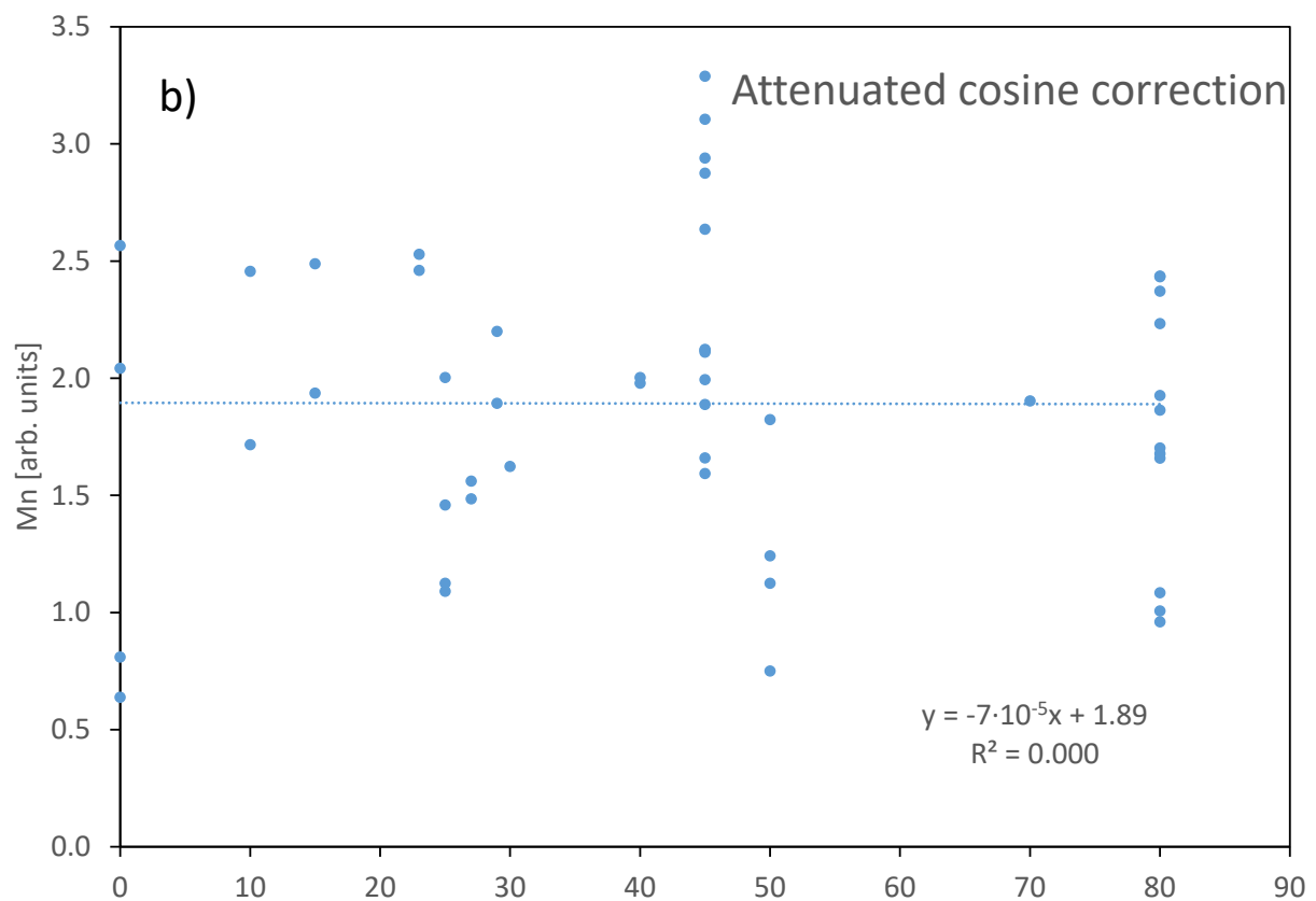
S5 Figure. Mn surface density versus surface inclination. a) without inclination correction, b) with correction using the "attenuated cosine" correction equation (see text).
