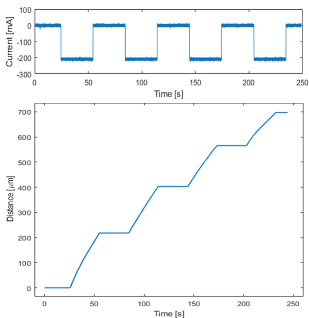
Figure S2. Raw data from LCMR calibration experiments. Top: step currents; bottom: the particle tracking result from video recorded through microscope.
