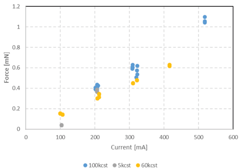
Figure S3. The master curve of force as a function of current for three silicone oils.
