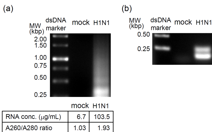
Figure S1. Purification of viral RNA from allantoic fluids of mock- or H1N1 IAV-infected chicken embryonated eggs. The viral RNA was checked by agarose gel electrophoresis for 20 \mu\text{L} purified samples (a) and RT-PCR products for segment 4 (b), as described in Materials and Methods. Any pellets after ultracentrifusion and enough RNA concentration for gel electrophoresis were not observed in the mock-infected sample.
