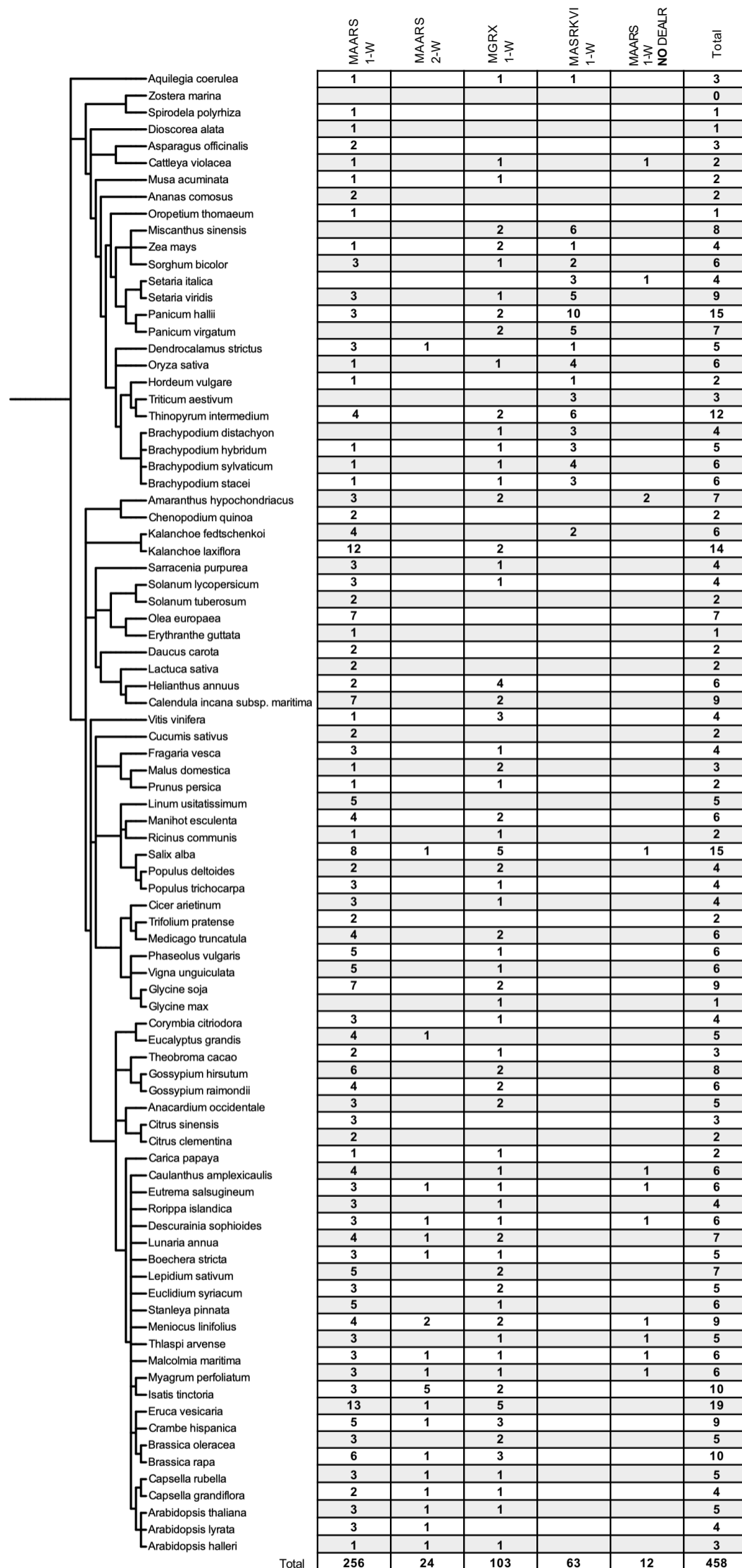
Figure S1. LEA3 Proteins in Higher plants by species. A plant species tree was generated using PhyloT and NCBI genomic reference numbers as described in the Materials and Methods. The five architectures for each LEA3 protein are listed. The total for each species listed in the right-hand column, and the total of each architecture are listed in the bottom row.
